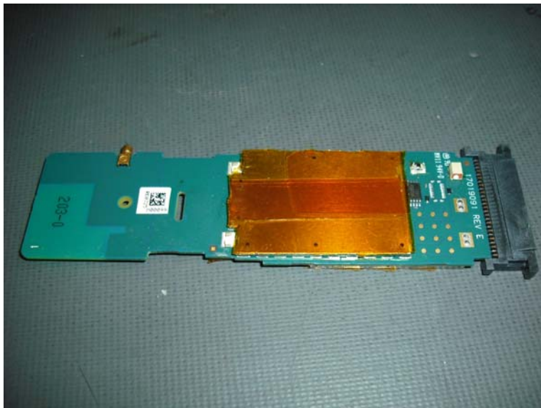
Bottom of PCB with Kapton Tape Installed
