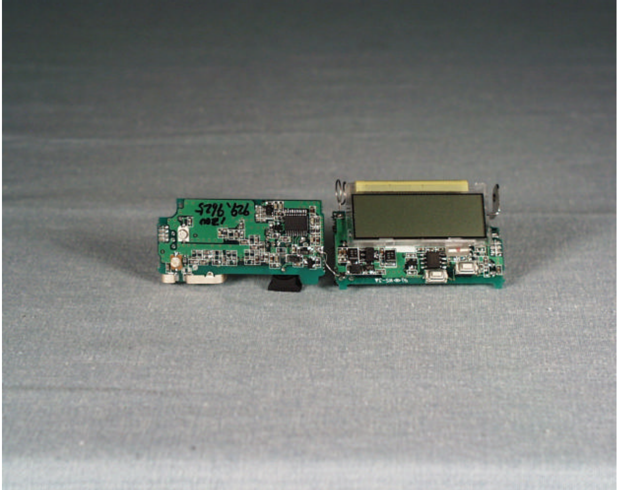
Component Side of the EPX-905N
