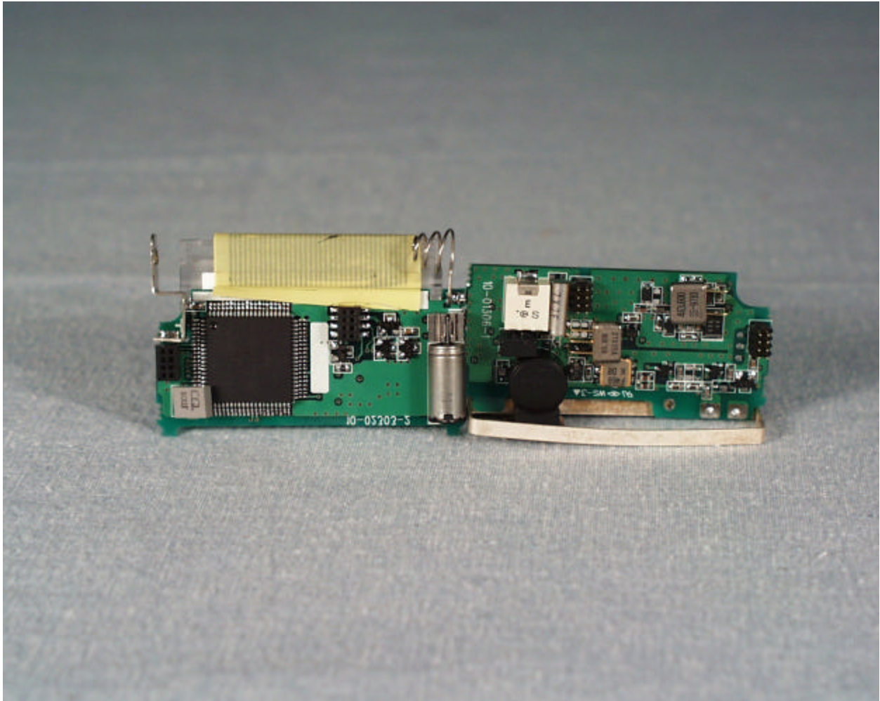
Alternate Component Side of the EPX-405N
