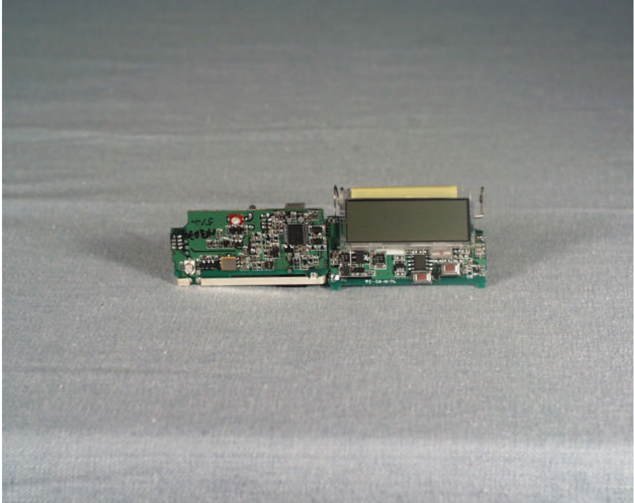
Component Side of the EPX-105N
