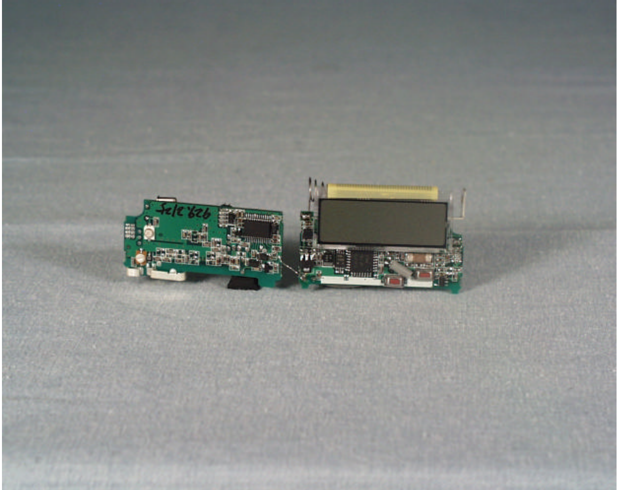
Component Side of the EFX-905N
