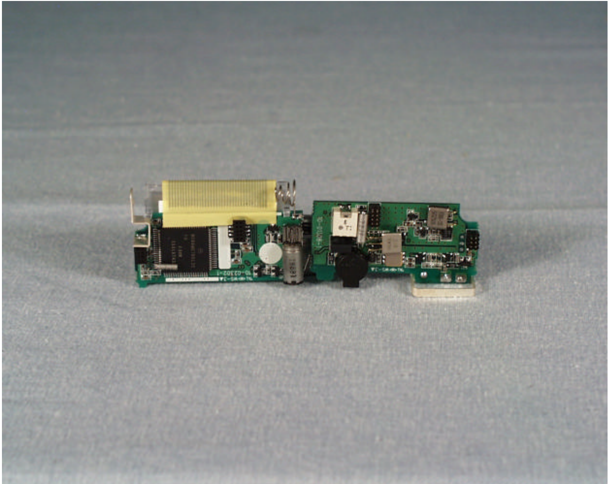
Alternate Component Side of the EFX-905N
