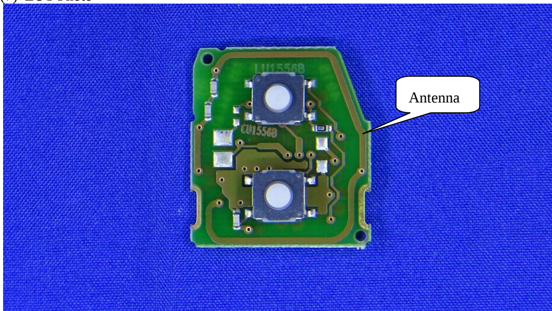
(7) EUT Photo
