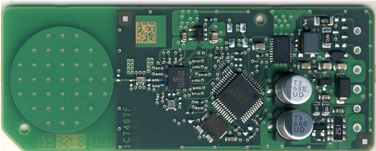
Picture 1: RSB19 PCB top photo
