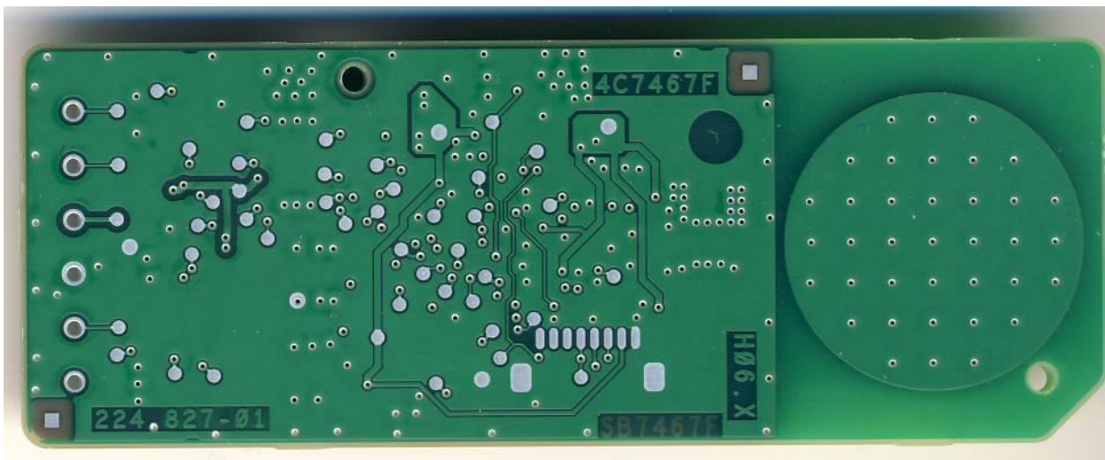
Picture 1: RSB19 PCB top photo
