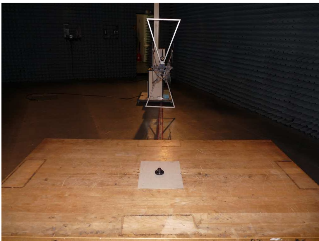
Photo 3: Test setup for radiated measurements (30 MHz to 1 GHz)
