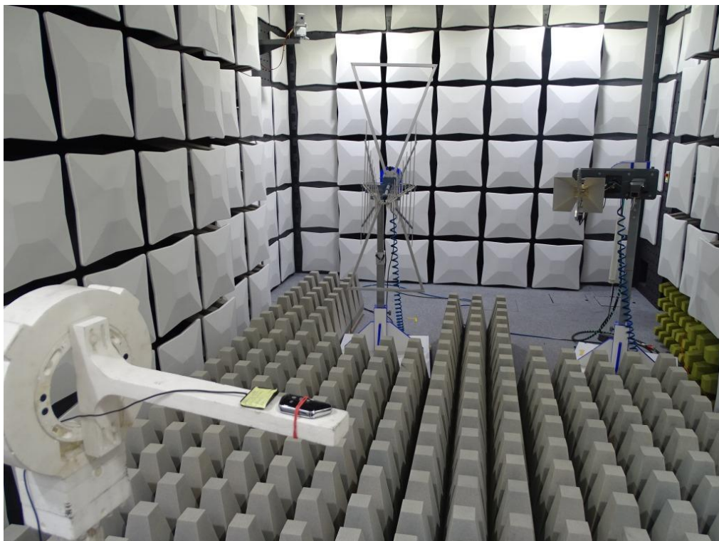
Photo 3: Test setup for radiated emissions measurements in fully-anechoic chamber (1 GHz to 7 GHz), right side view, 3 m measurement distance
