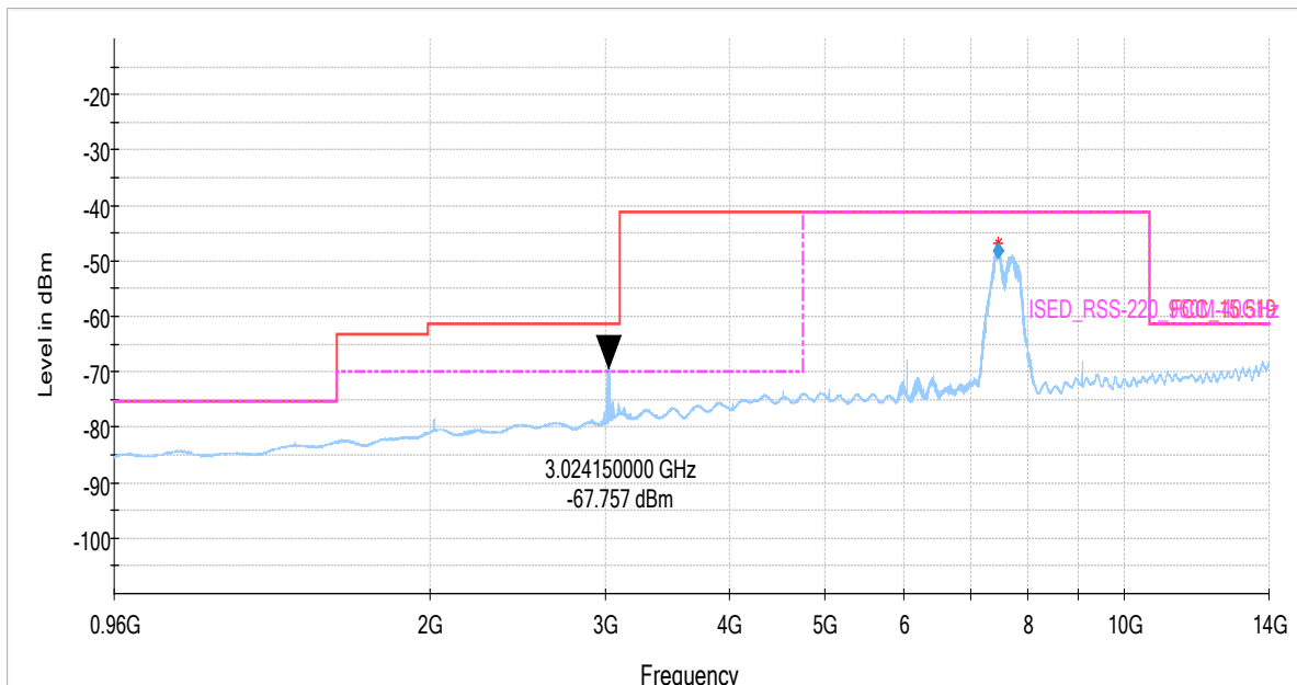
960 MHz – 14 GHz
