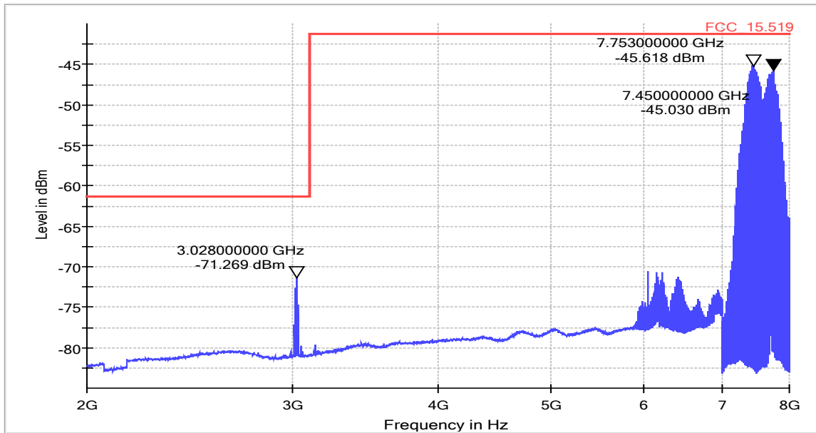
TX, 7560 MHz, conducted measurement at antenna connector
