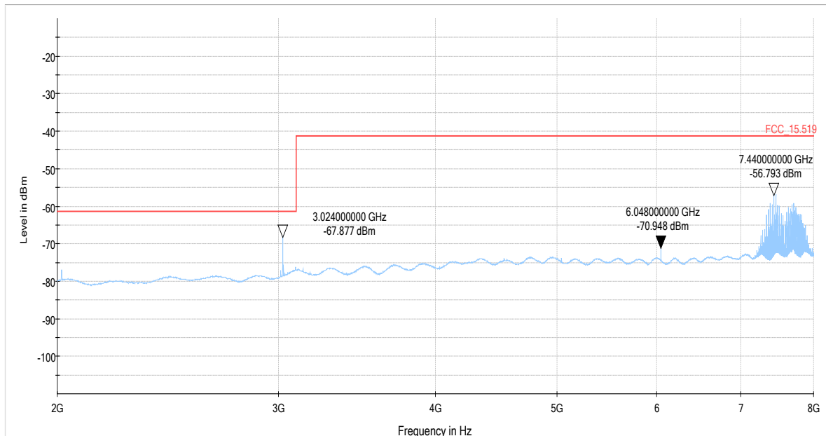
TX, 7560 MHz, radiated measurement with antenna connector terminated with 50 Ohm
