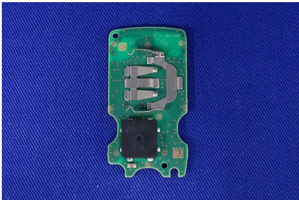
(32) EUT Photo
