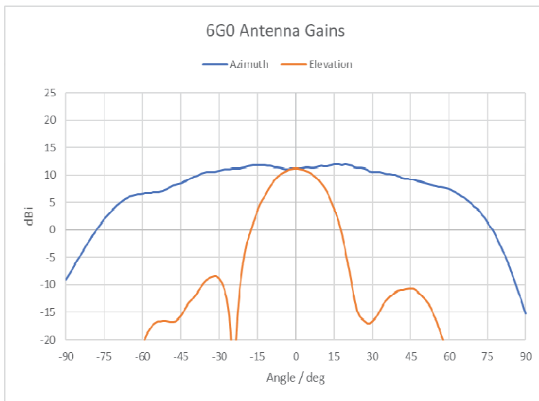
Tx1, Tx2 and Tx3 antenna characteristics in azimuth and in elevation. The peak gain is approx. 11 dBi.
