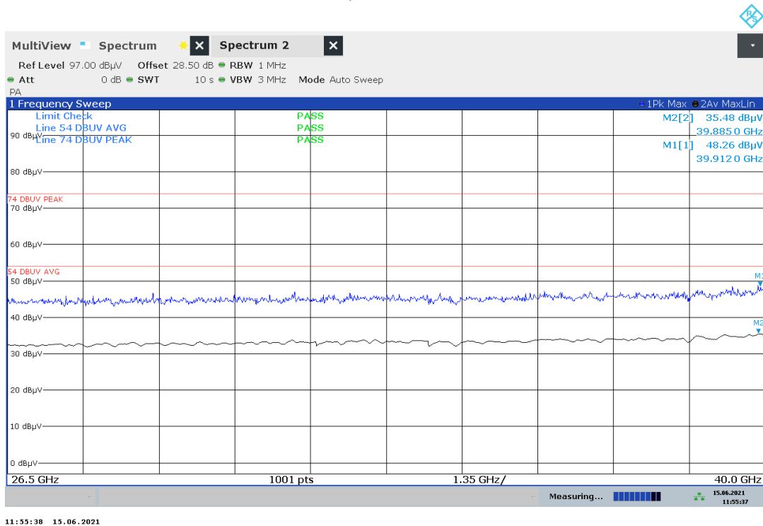
Plot no. 18: radiated emissions 26.5 GHz – 40 GHz, polarization vertical / horizontal
