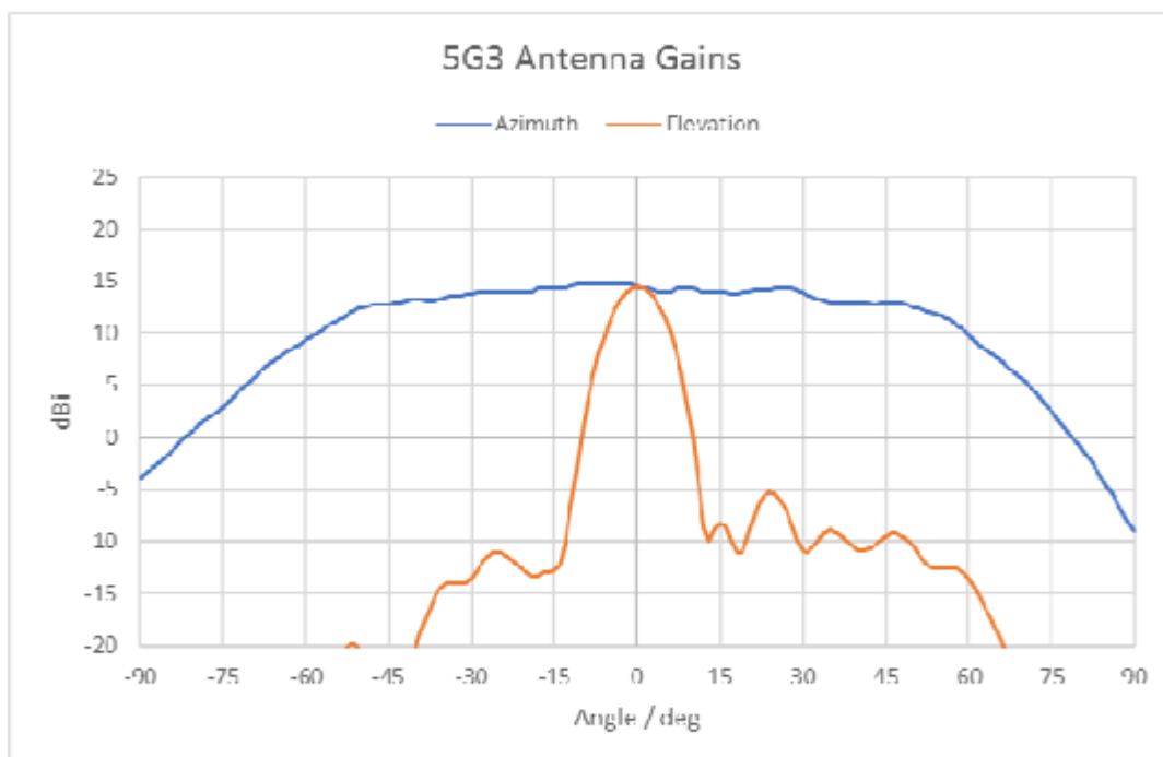
Antenna characteristics in azimuth and in elevation. The peak gain is approx. 15 dBi.
