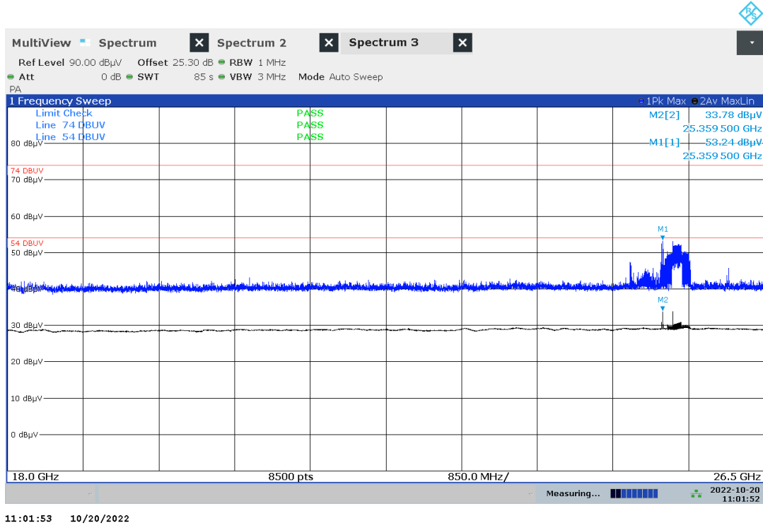
Plot no. 16: radiated emissions 18 GHz – 26.5 GHz, polarization vertical / horizontal, mode 0
