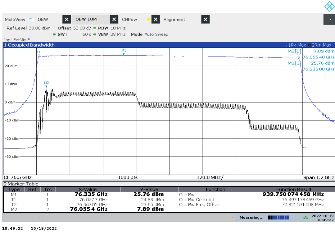
Plot no. 7: OBW, Peak detector, Mode 1
