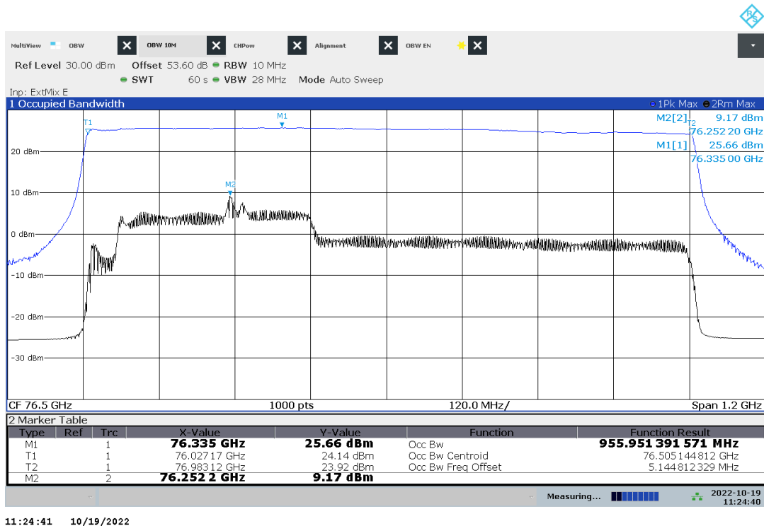
Plot no. 8: OBW, Peak detector, Mode 2
