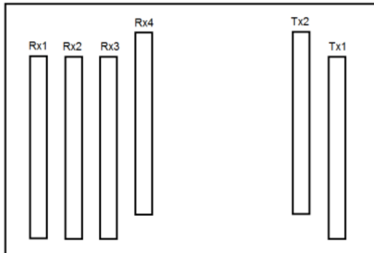
Illustration of Tx and Rx antennas inside the EUT. Each antenna consists of a linear patch array with horizontal polarisation.
