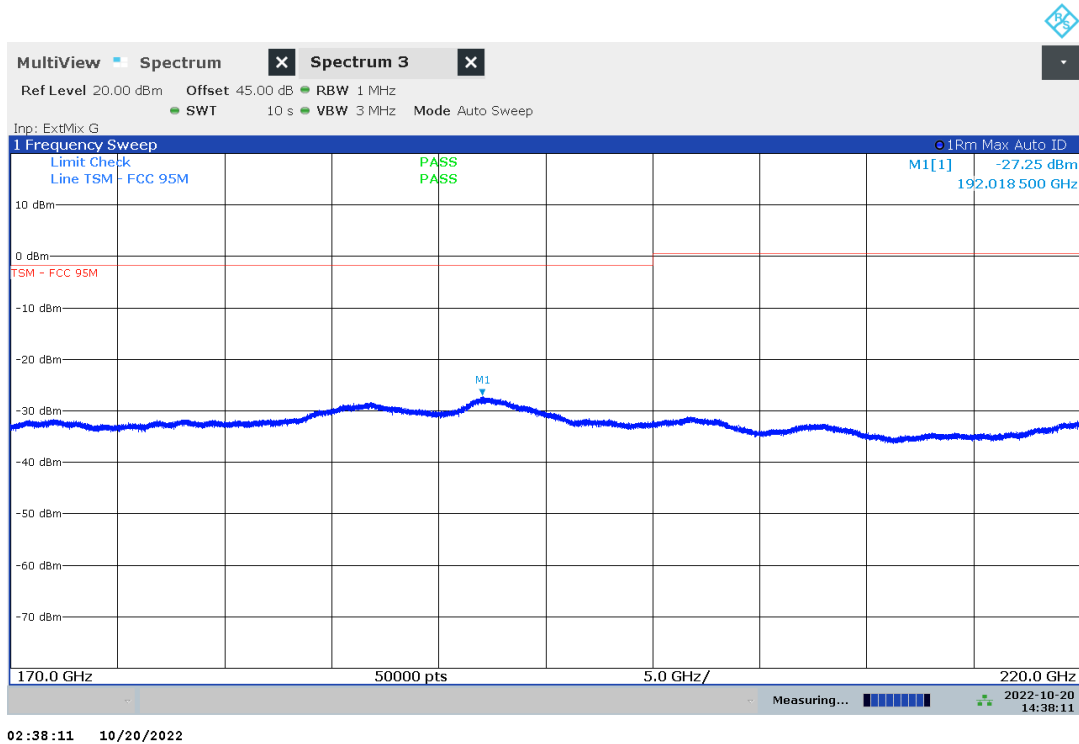
Plot no. 23: radiated emissions 170 GHz – 220 GHz, polarization vertical / horizontal, mode 0
