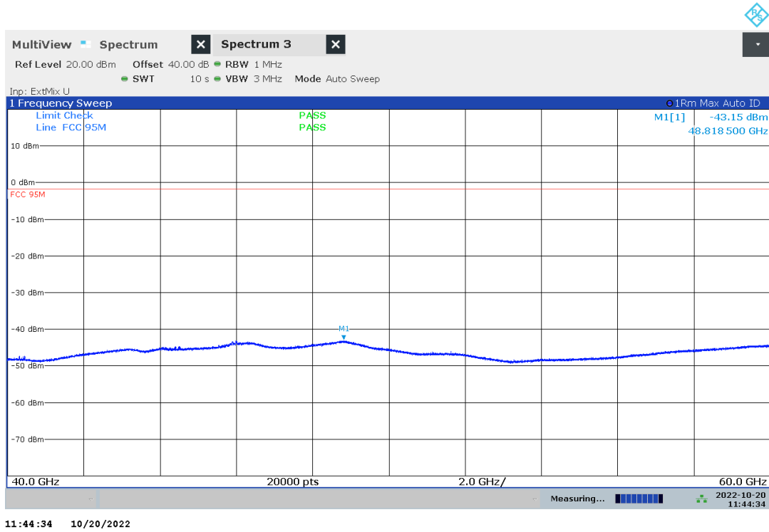
Plot no. 18: radiated emissions 40 GHz – 60 GHz, polarization vertical / horizontal, mode 0
