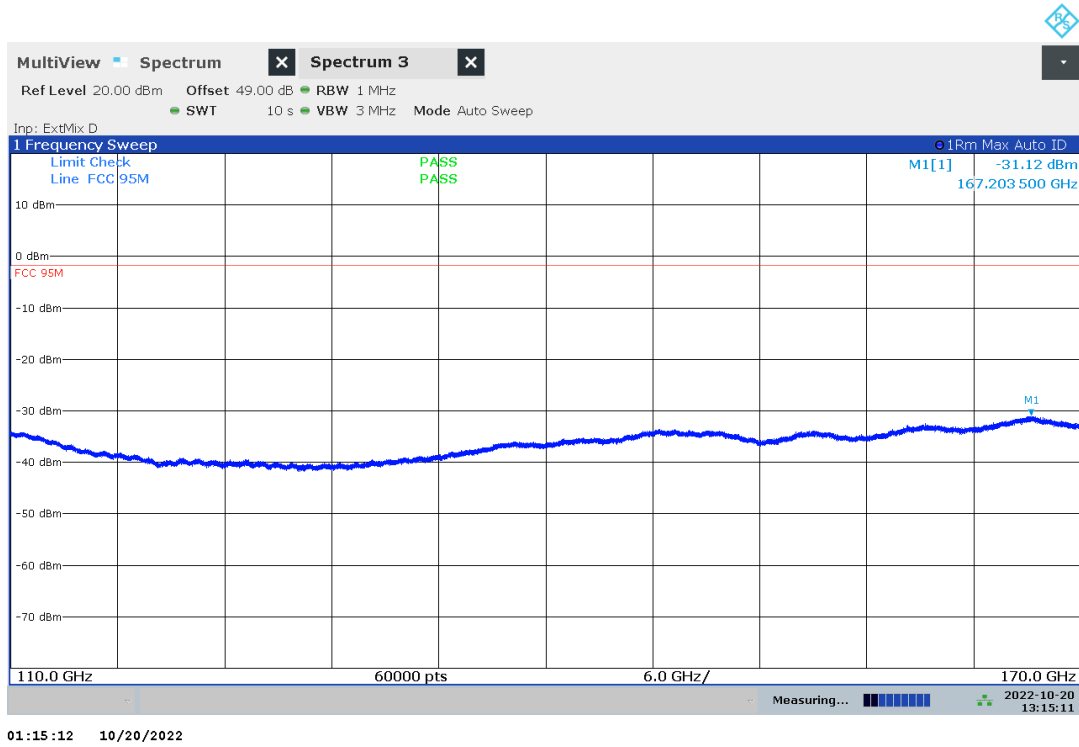
Plot no. 22: radiated emissions 110 GHz – 170 GHz, polarization vertical / horizontal, mode 0
