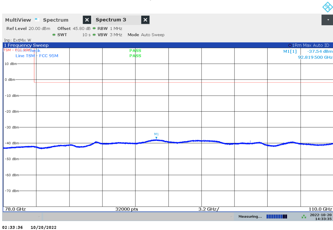
Plot no. 21: radiated emissions 78 GHz – 110 GHz, polarization vertical / horizontal, mode 0
