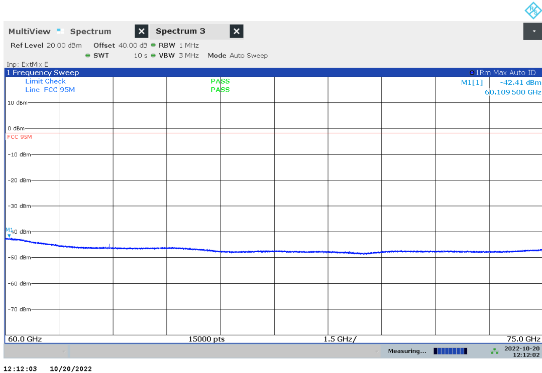
Plot no. 19: radiated emissions 60 GHz – 75 GHz, polarization vertical / horizontal, mode 0
