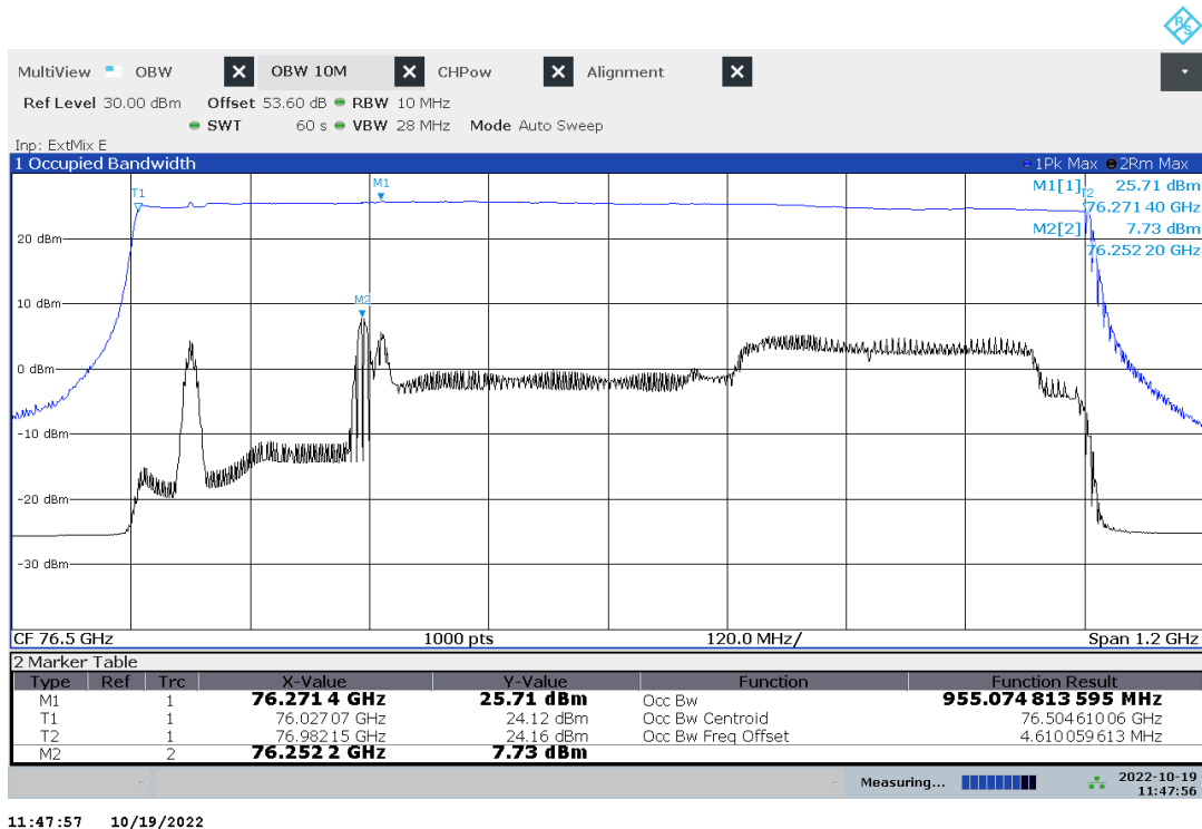
Plot no. 12: OBW, Peak detector, Mode 6
