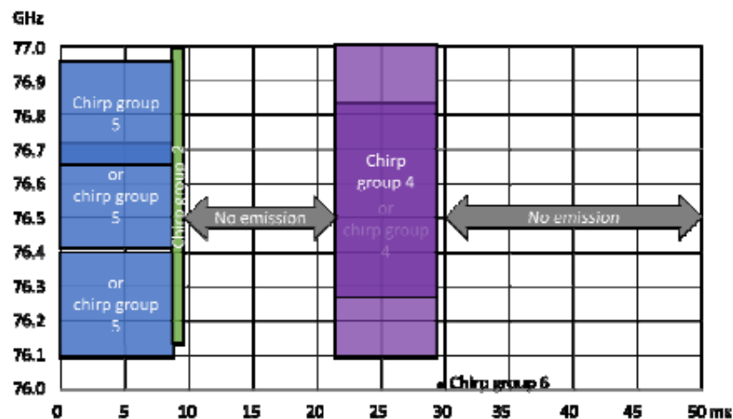
Illustration of time dependent modulation within one radar cycle.
