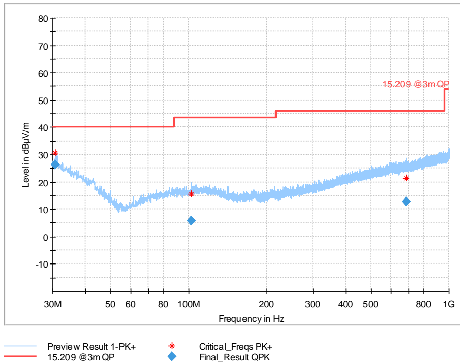
Plot no. 14: radiated emissions 30 MHz – 1 GHz, polarization vertical / horizontal, mode 0
