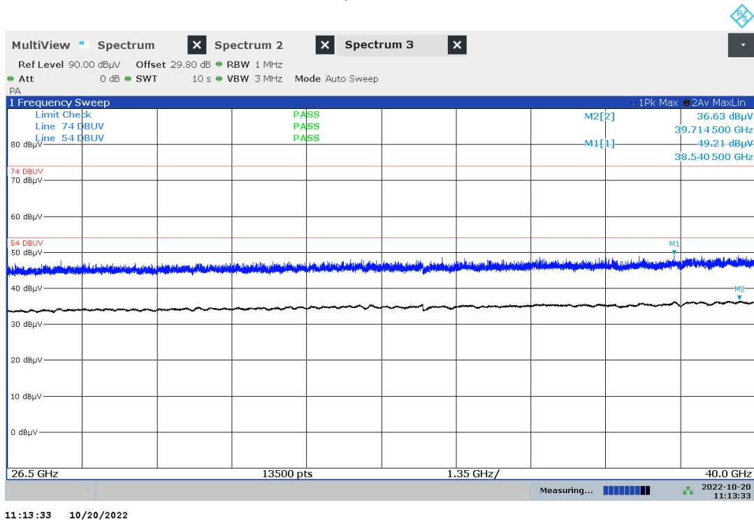
Plot no. 17: radiated emissions 26.5 GHz – 40 GHz, polarization vertical / horizontal, mode 0
