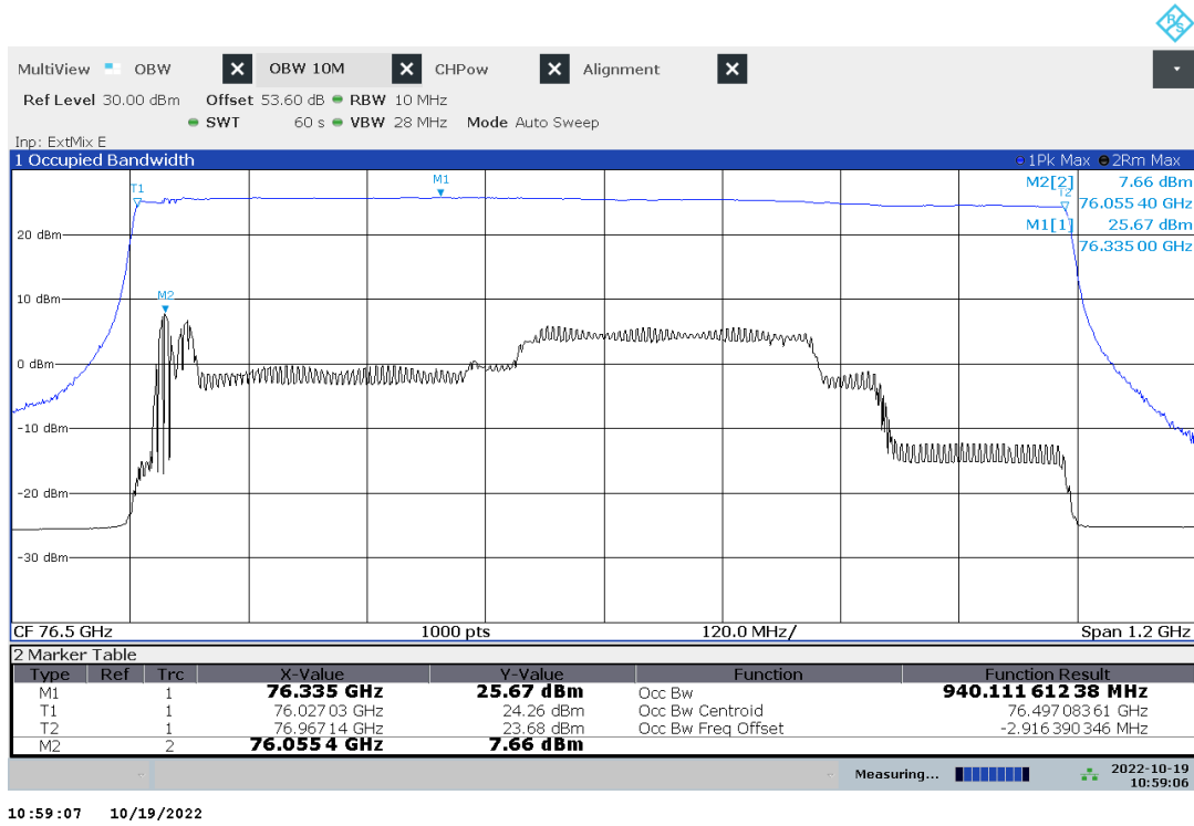
Plot no. 9: OBW, Peak detector, Mode 3
