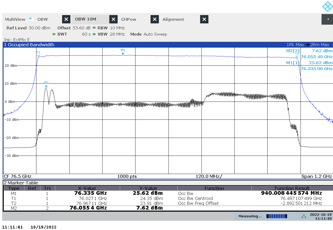
Plot no. 11: OBW, Peak detector, Mode 5
