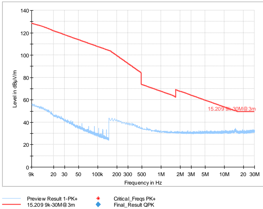
Plot no. 13: radiated emissions 9 kHz – 30 MHz, loop antenna, mode 0
