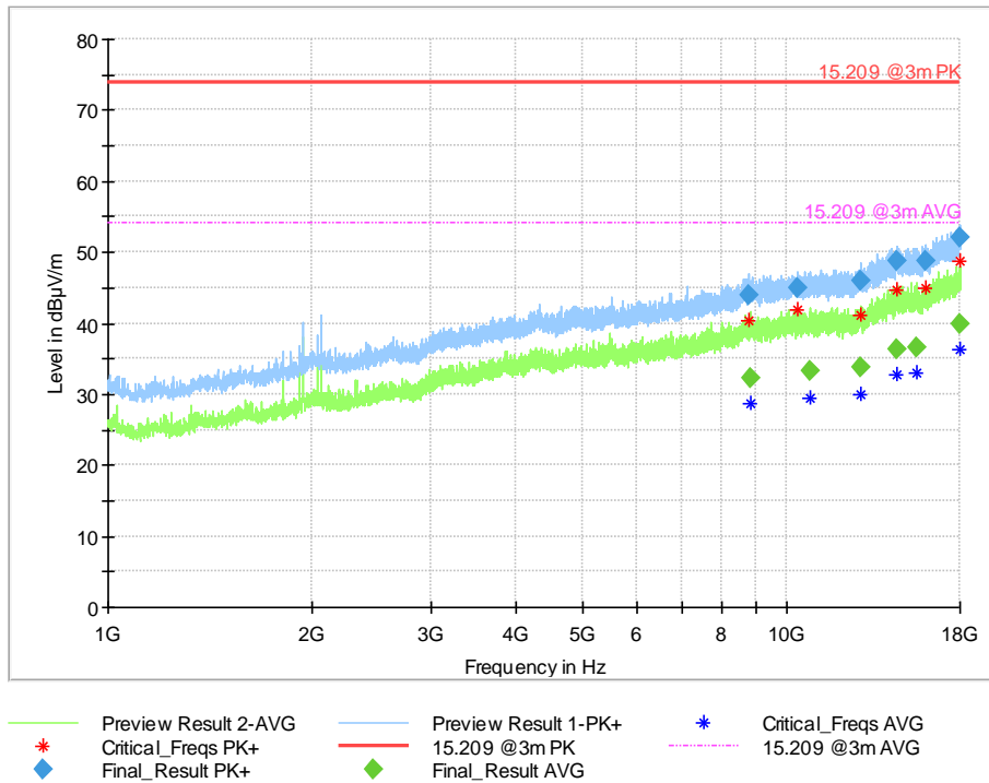
Plot no. 15: radiated emissions 1 GHz – 18 GHz, polarization vertical / horizontal, mode 0
