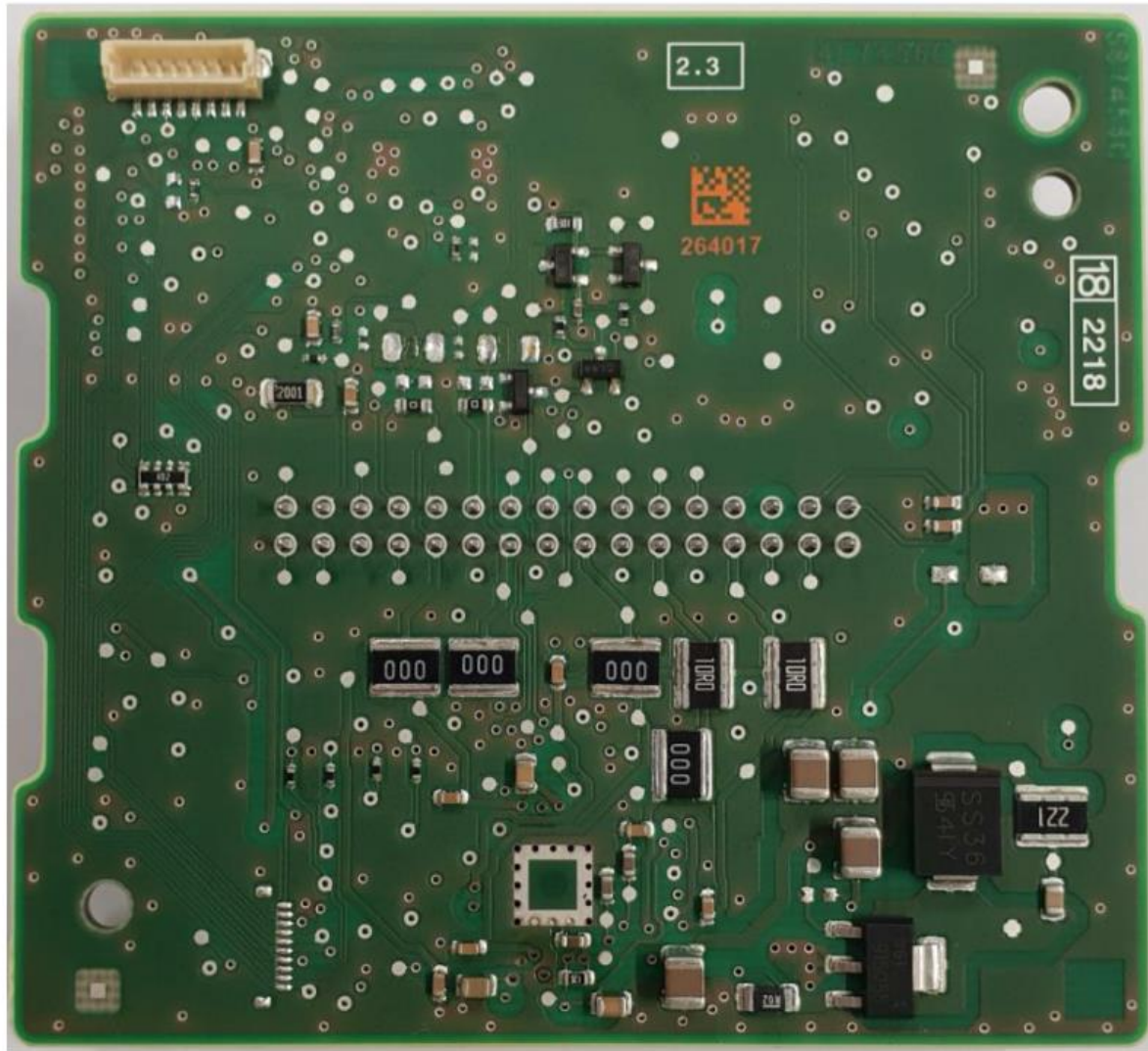
Mod. 013854, PCB bottom view:
