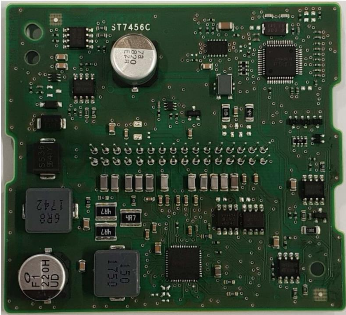
Mod. 013854, PCB top view
