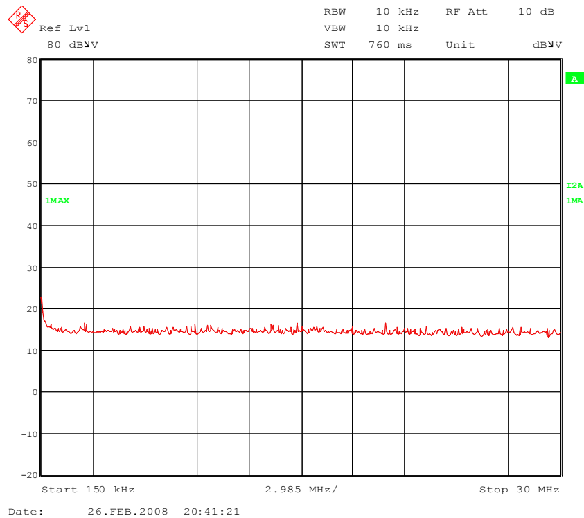
72572vw_H2.wmf: Radiated emissions from 150 kHz to 30 MHz
