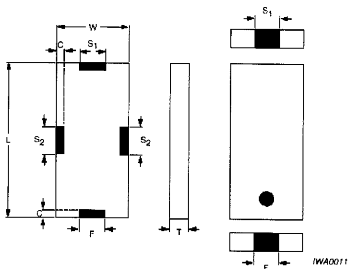
Fig. 1. Component outline.
