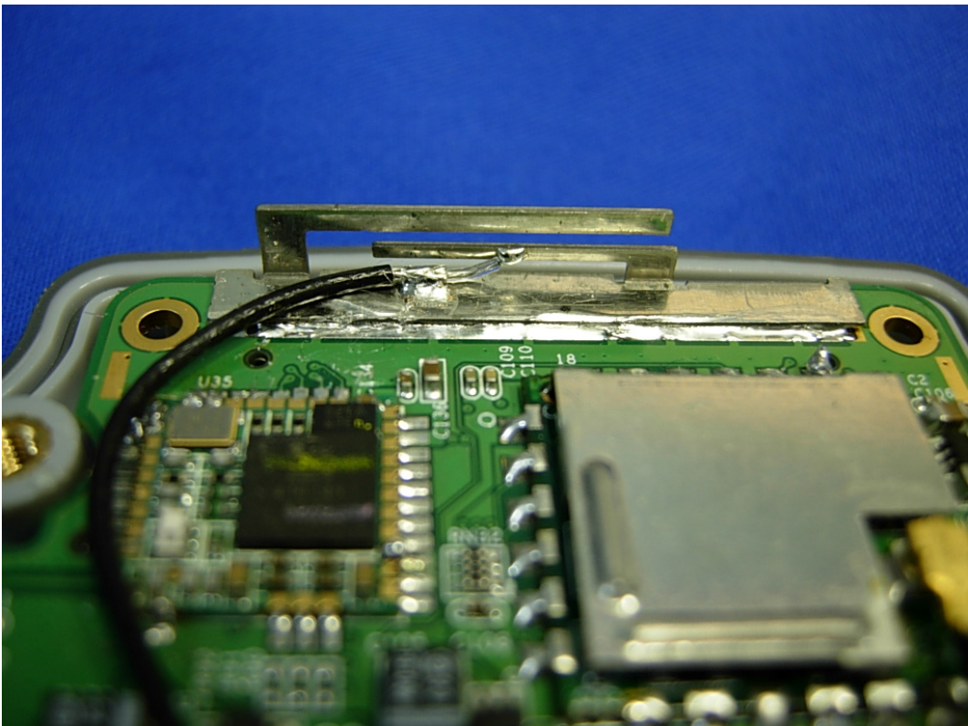
(12) EUT Photo (WLAN Antenna)
