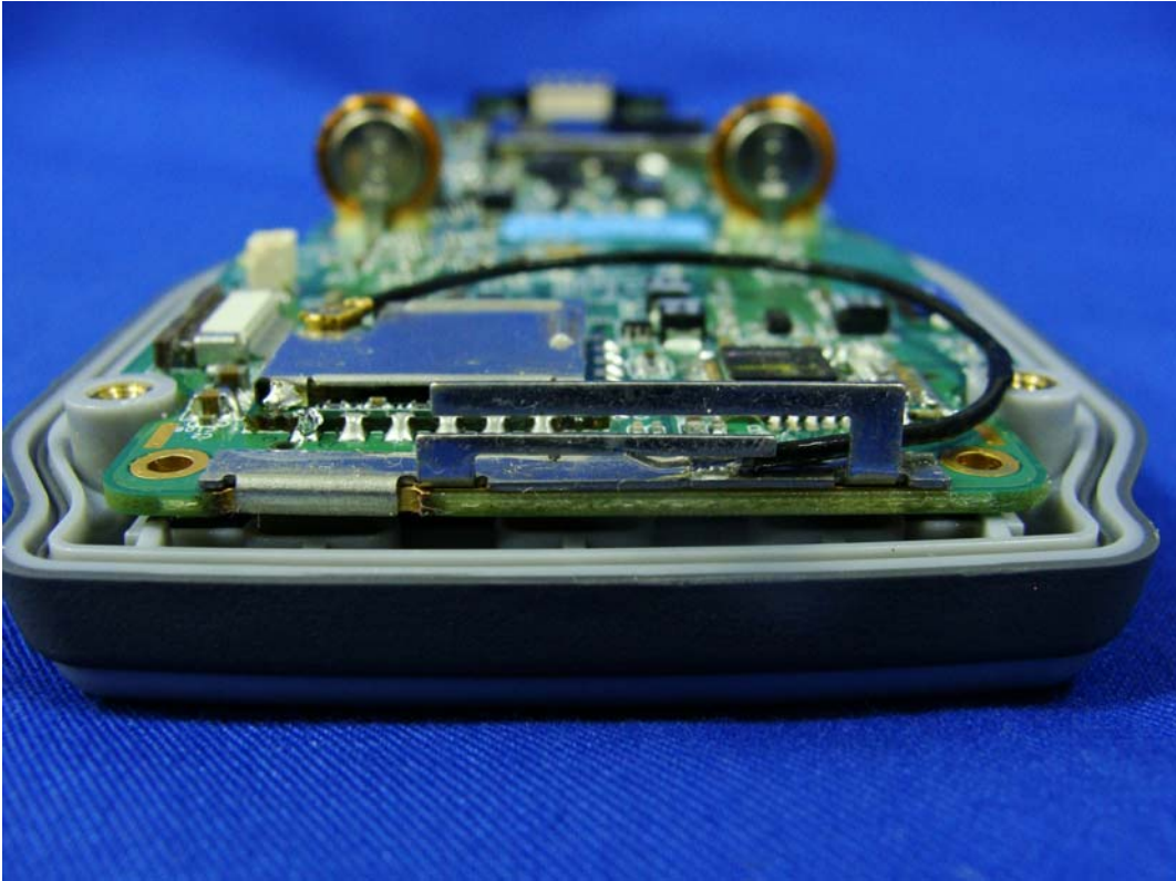
(11) EUT Photo (WLAN Antenna)
