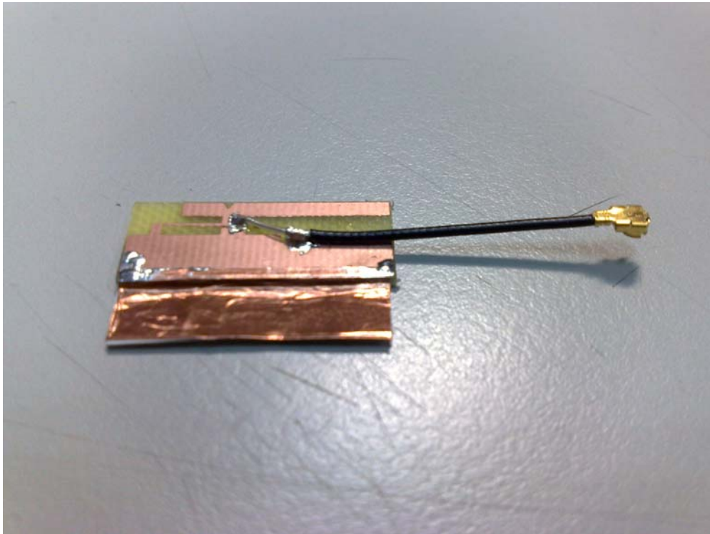
(6) EUT Photo (Antenna- JI-HAW / 69-70003-002 )
