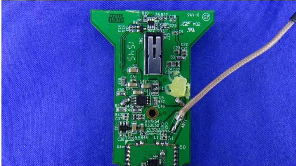
(11) EUT Photo
