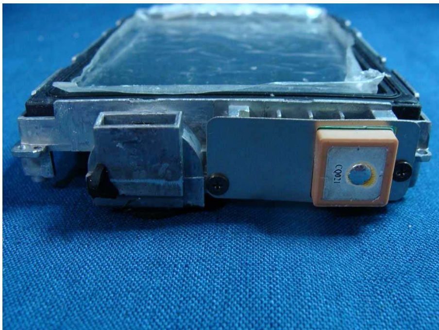
(28) EUT Photo
