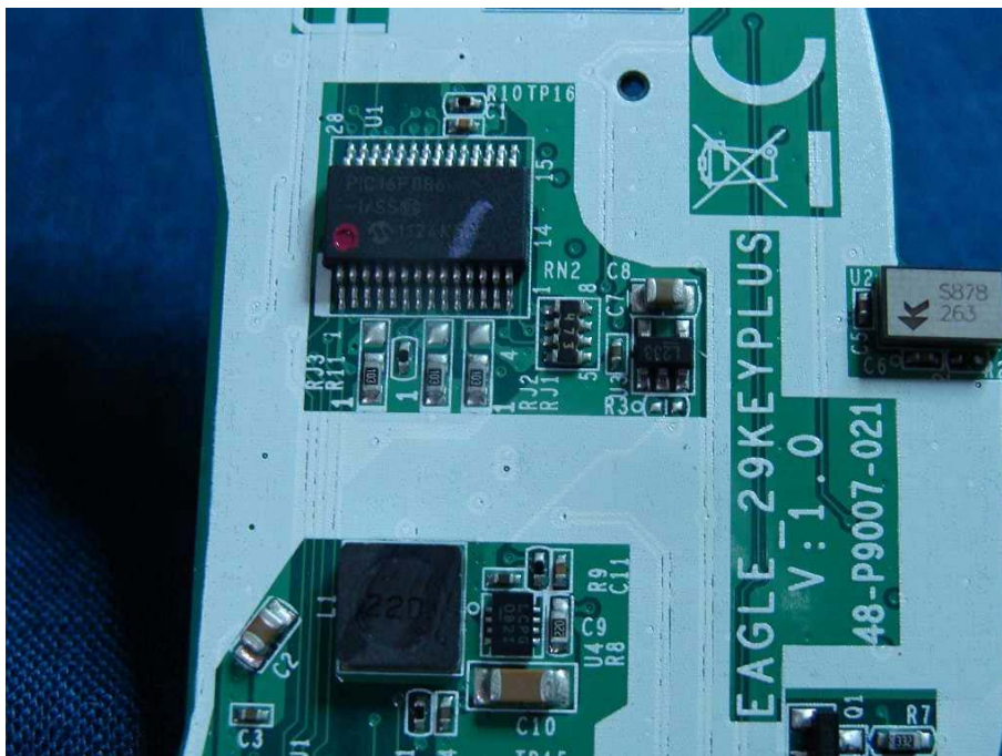
(32) EUT Photo
