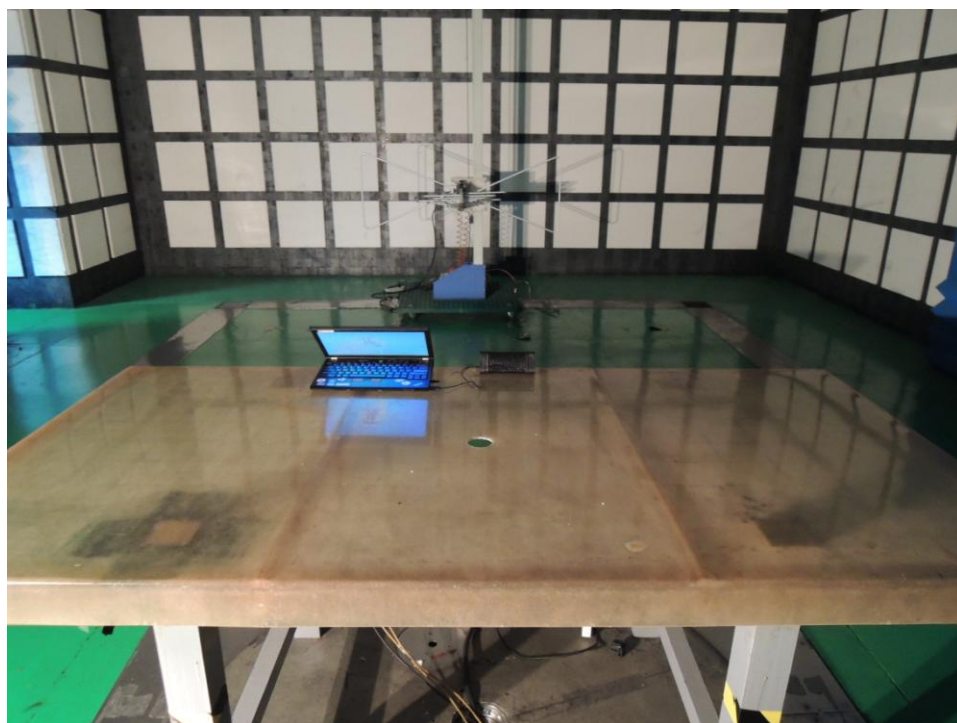
Spurious radiated emission (30MHz-1000MHz)
