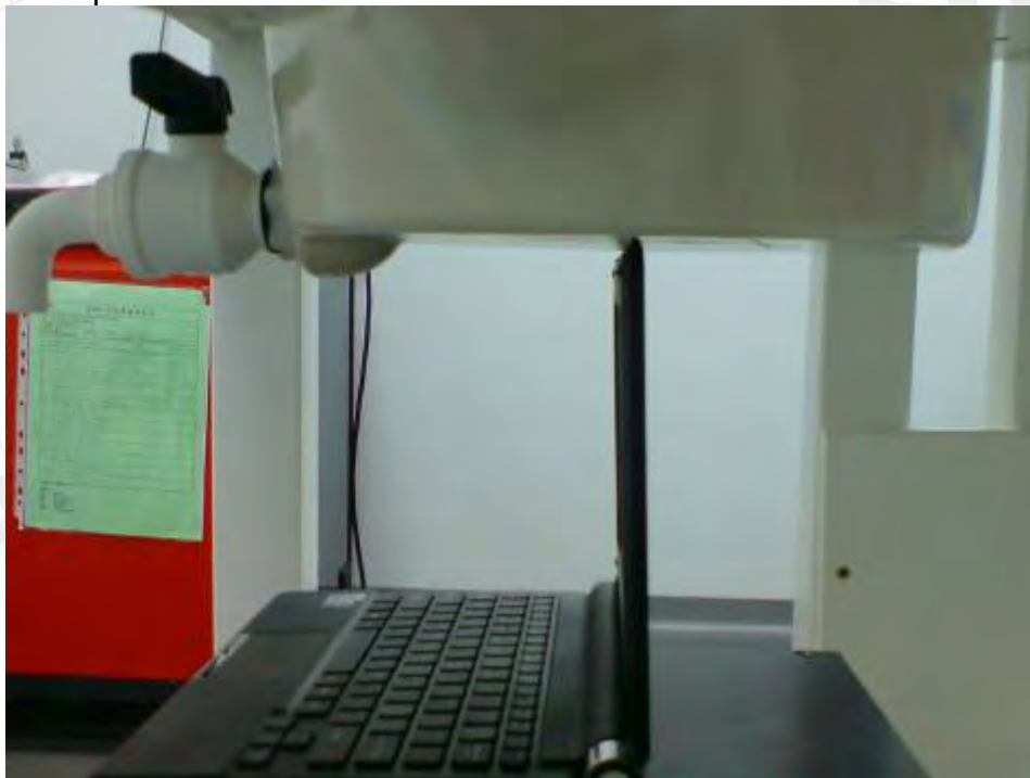
Fig.6 Top side of EUT is paralleled with flat phantom, and contact with flat phantom.
