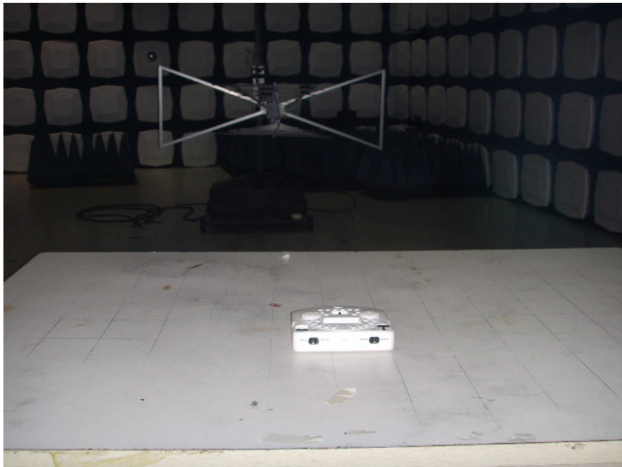
Test Setup – Back View
