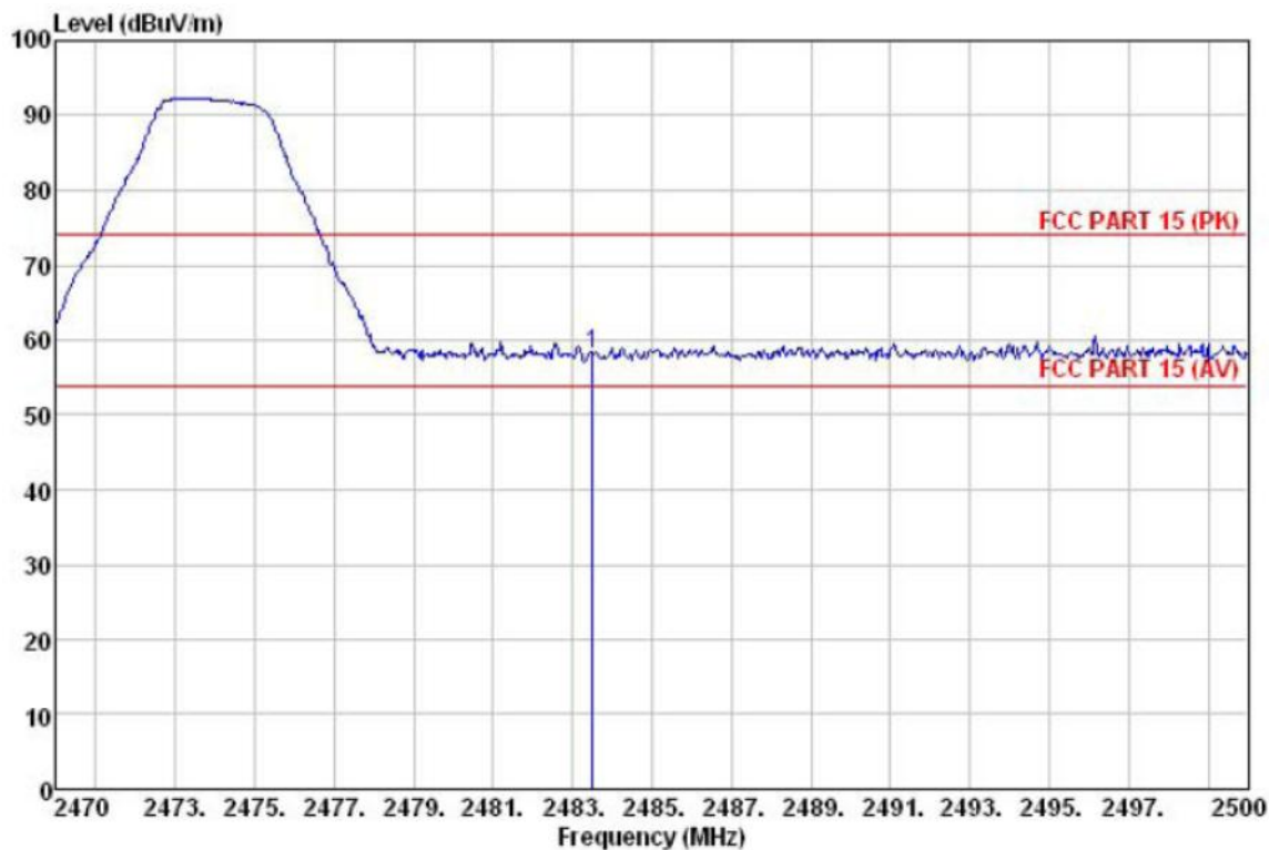
Radiated measurement
