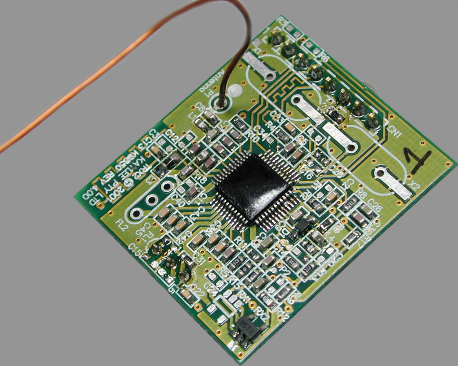
Internal Radio Mod Front View
