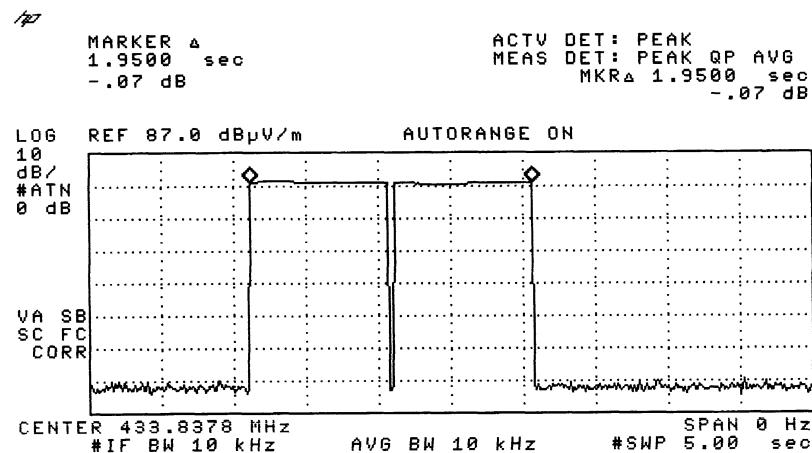
Periodic operation [FCC 47CFR15.231a] Figure F
