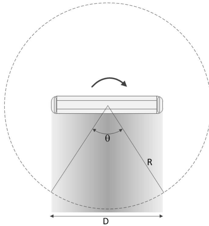
Figure 1 Top-view figure showing the antenna and the rotational direction. The beam is shown in gray, with a width D equivalent to the antenna width and spanning an angle \theta at a distance of R meters.
