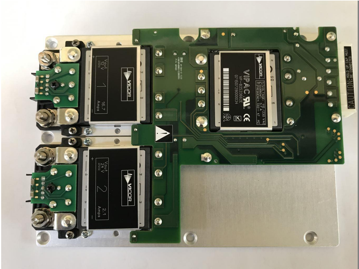
Power Supply Unit Module: Switch Mode Circuit Card Assembly
