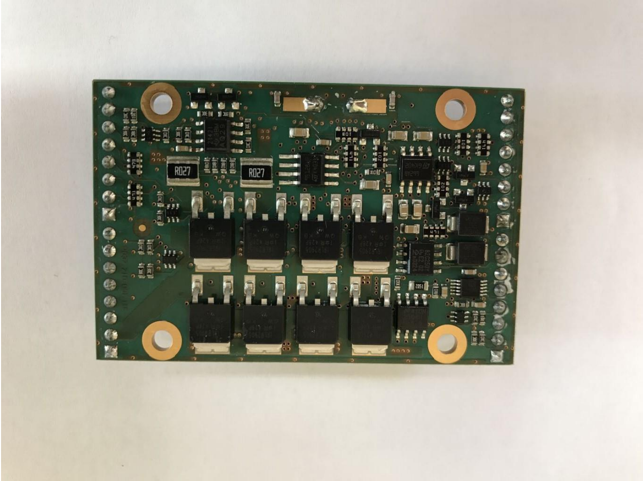
Motor Controller Module: Motor controller Circuit Card Assembly (Top)
