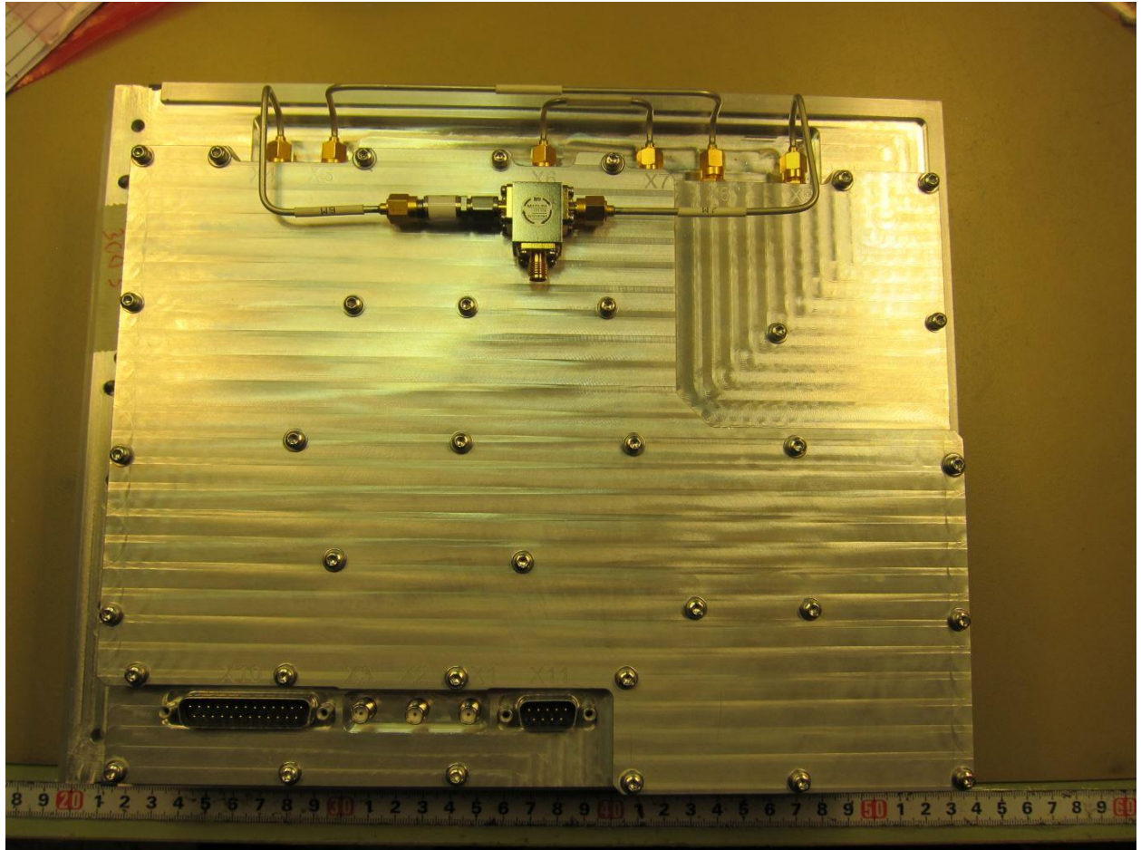
Transceiver Module
