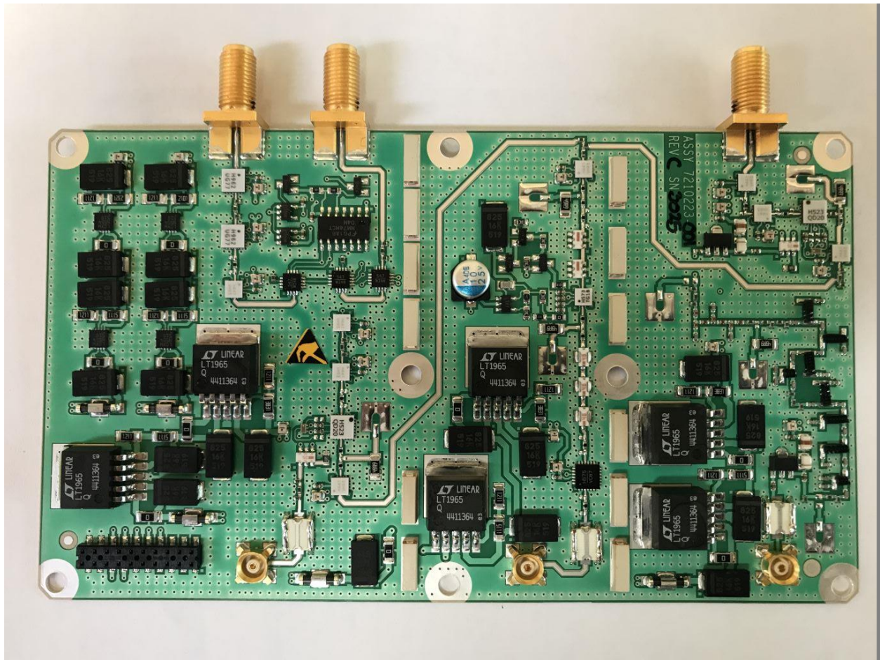
Transceiver Module: Radio Frequency Circuit Card Assembly (Top)
