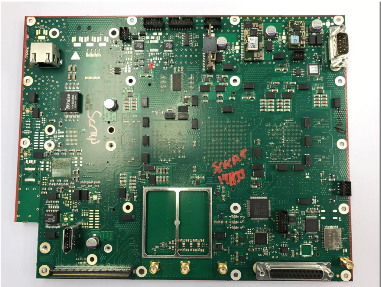
Processing Module: Processing Circuit Card Assembly (Top)
