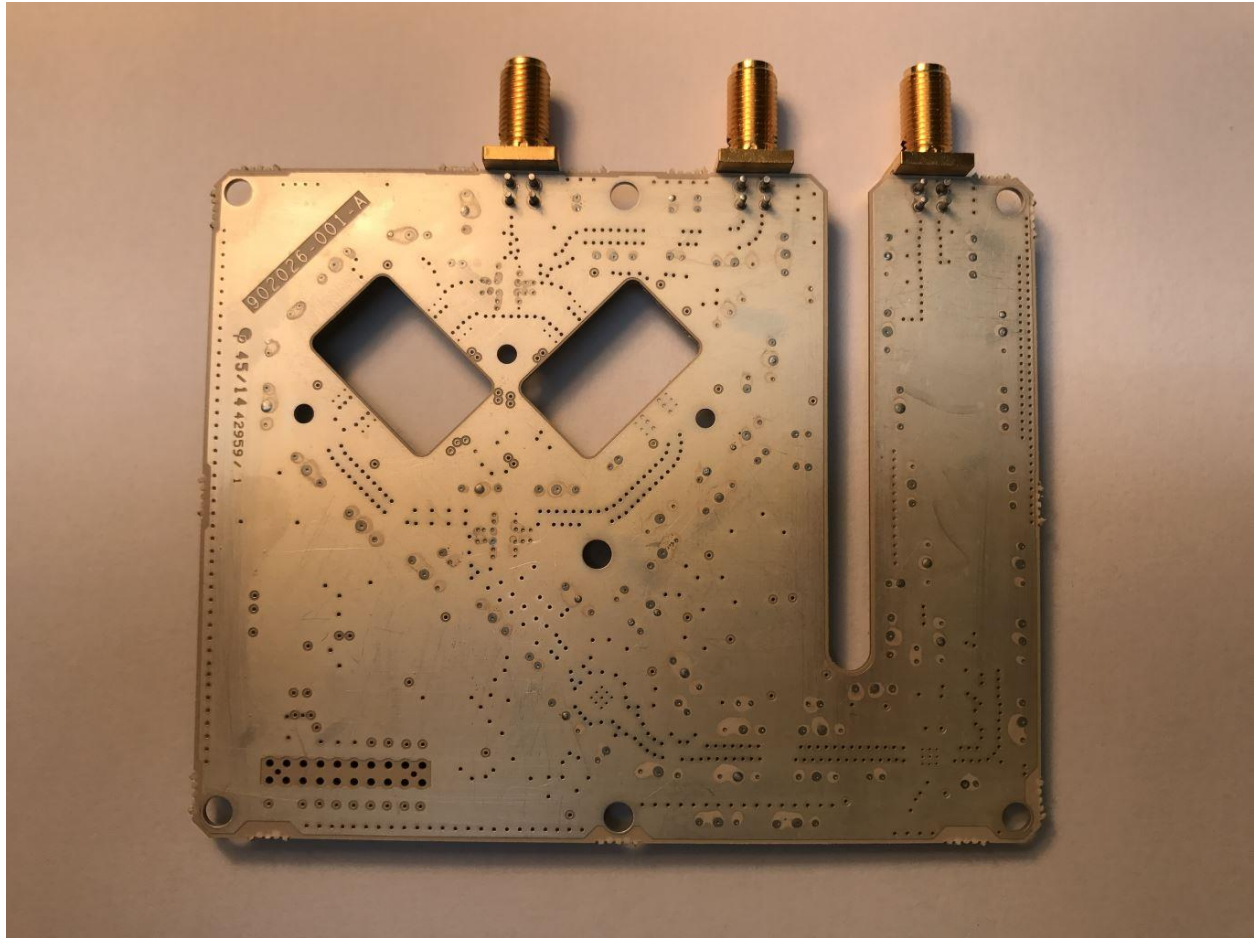
Transceiver Module: Solid State Power Amplifier Circuit Card Assembly (Bottom)
