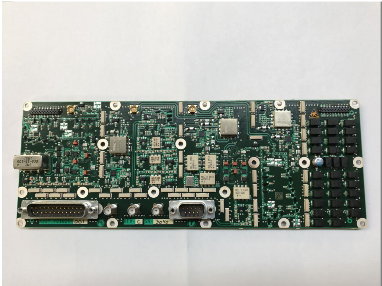
Transceiver Module: Intermediate Frequency Circuit Card Assembly (Top)
