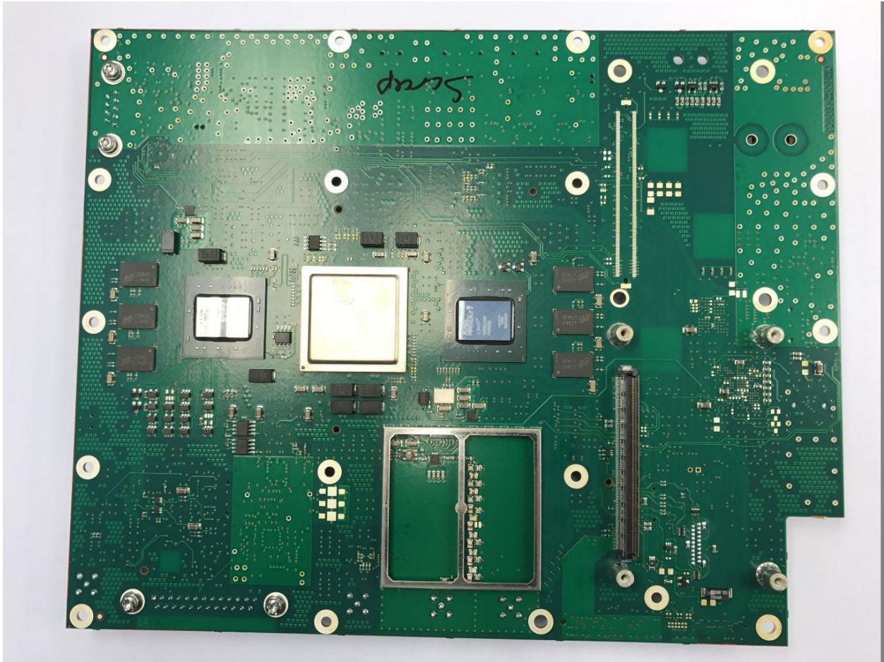
Processing Module: Processing Circuit Card Assembly (Bottom)
