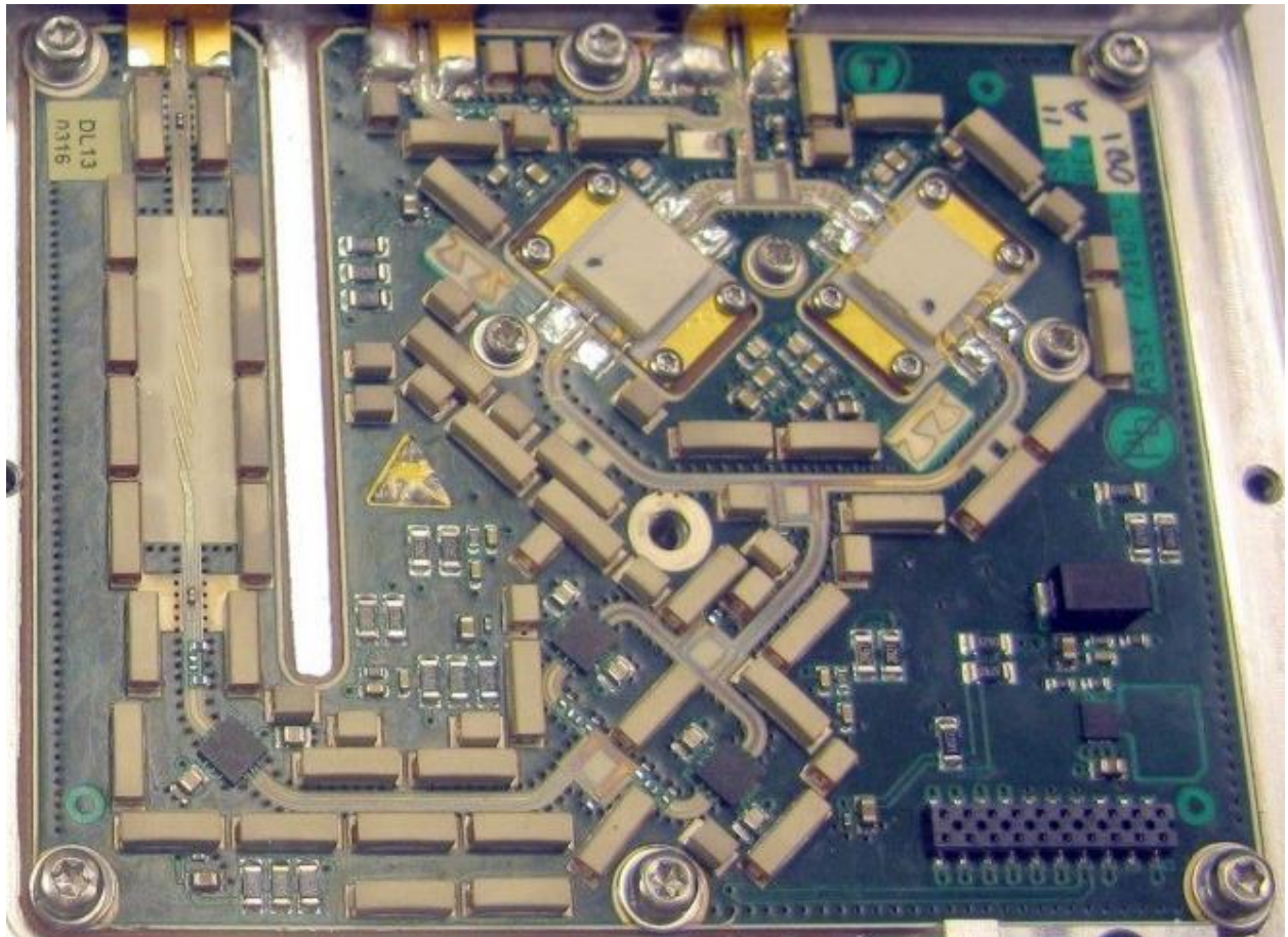
Transceiver Module: Solid State Power Amplifier Circuit Card Assembly (Top)
