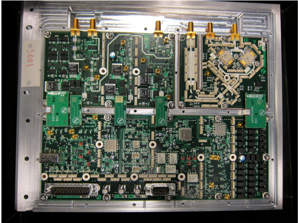
Transceiver Module: Inside
