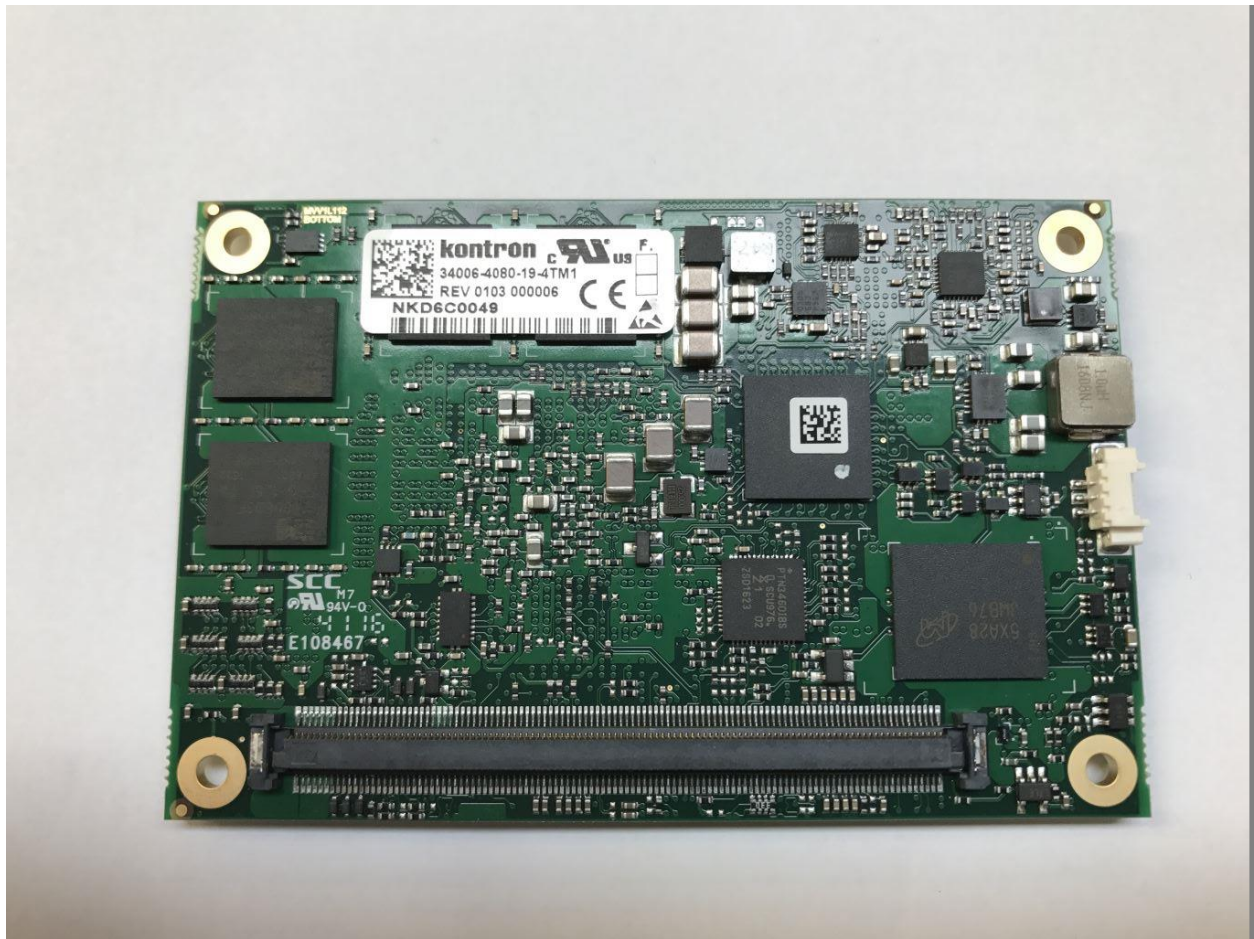
Processing Module: Computer Circuit Card Assembly (Top)
