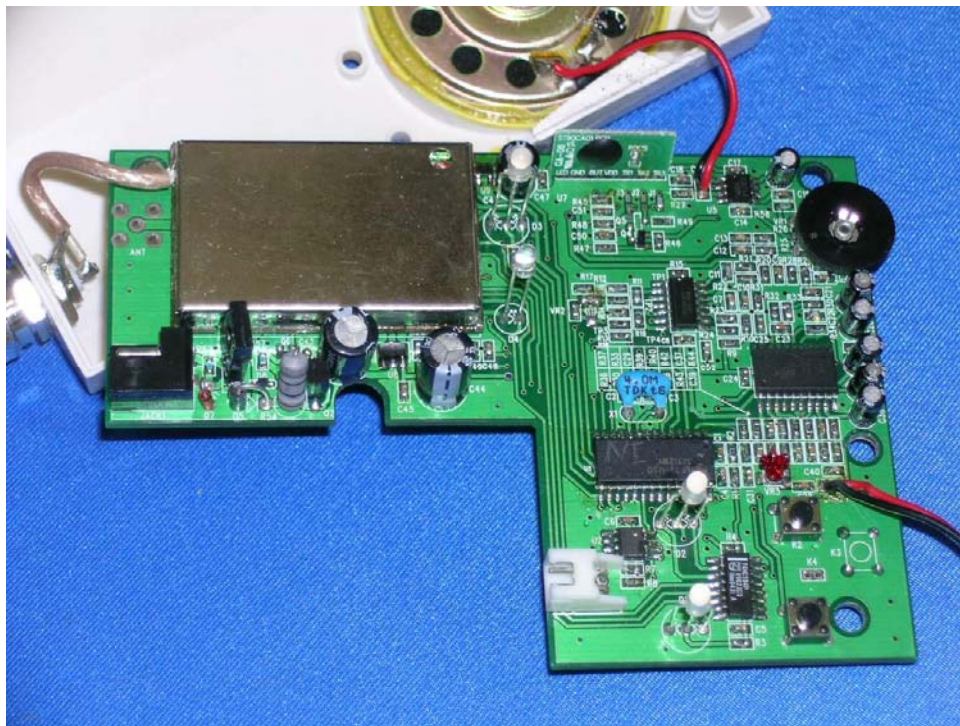
Intercom Unit Main PCB comp side (View 1)
