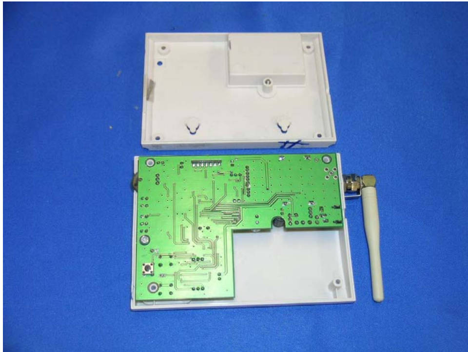
Intercom Unit assembly
