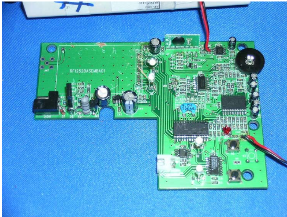
Intercom Unit Main PCB comp side (View 2)
