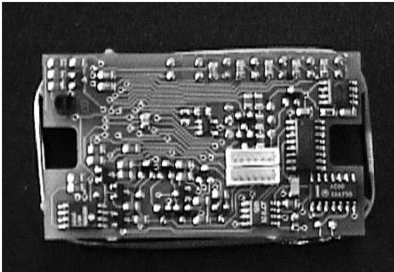
Figure 1 - PCB Side 1
