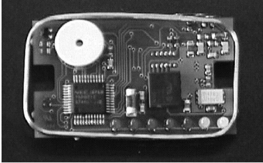
Figure 2 - PCB Side 2
