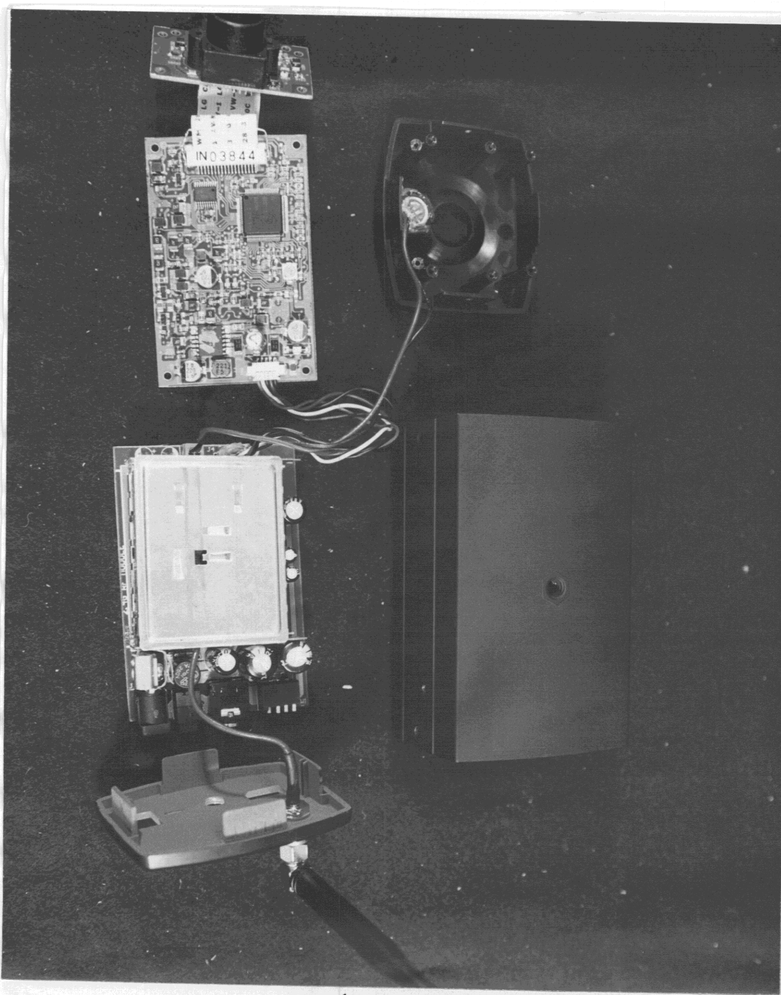
FCC ID : N9AWS-040-AN E.U.T : 2.4GHz Wireless Security System Internal View of EUT
