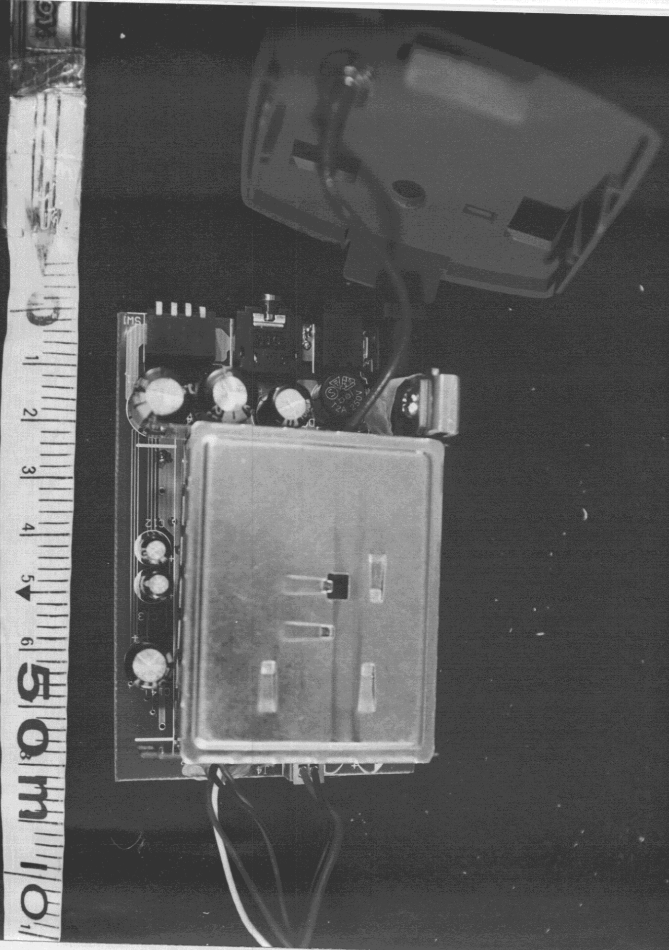
One Side View 1 of PCB 1
