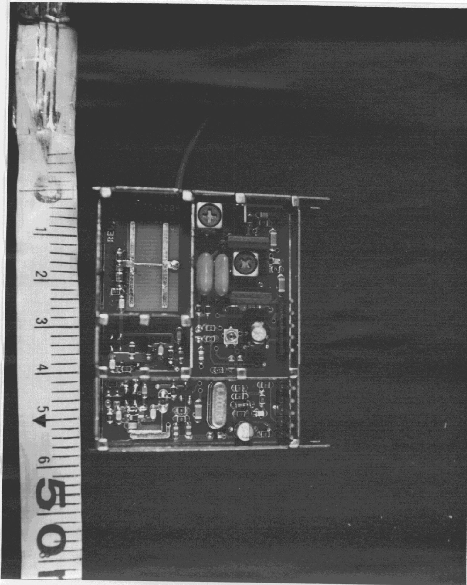
FCC ID : N9AWS-040-AN E.U.T : 2.4GHz Wireless Security System One Side View Of RF Module's Board
