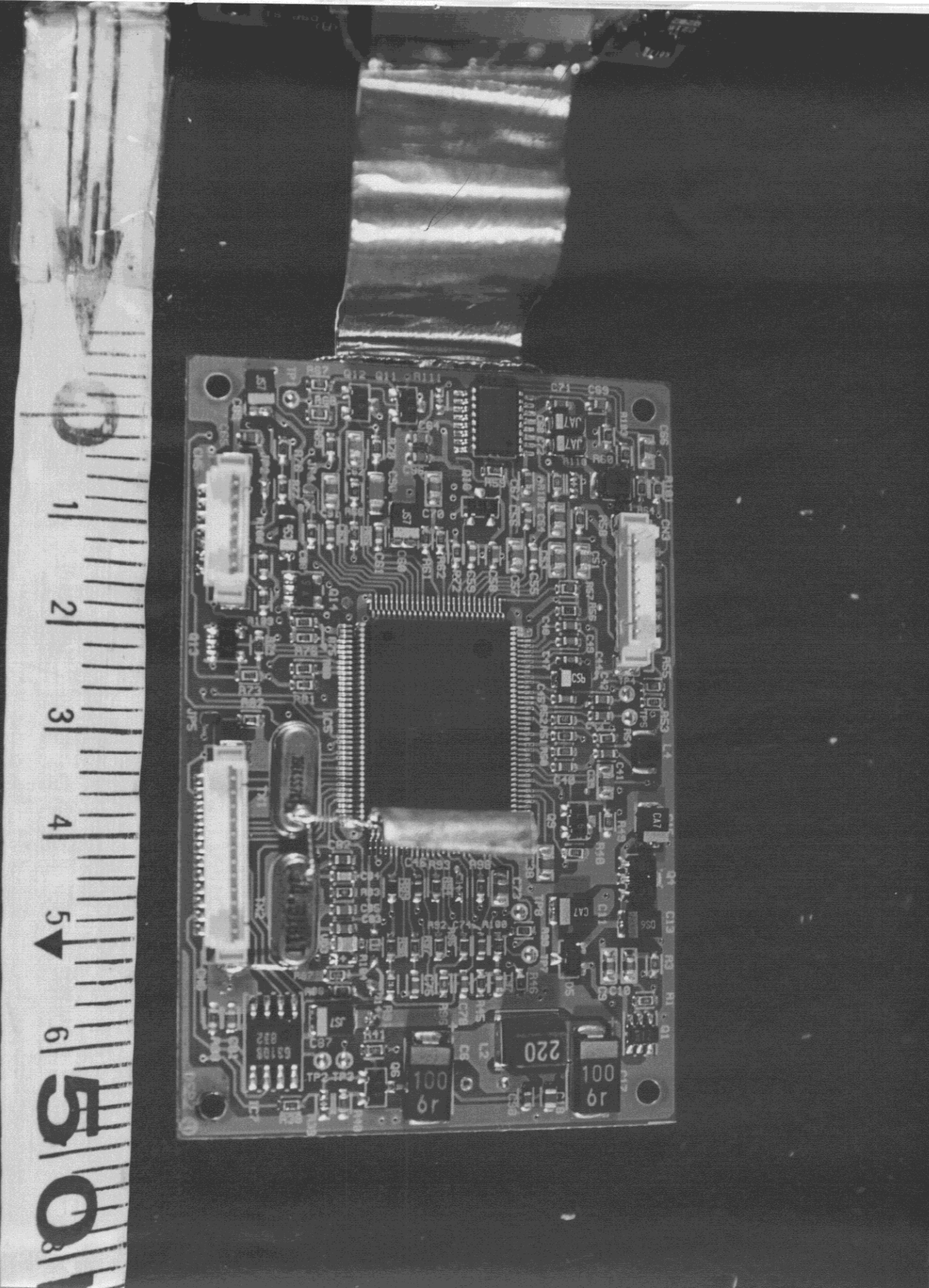
One Side View 2 Of Main Board
