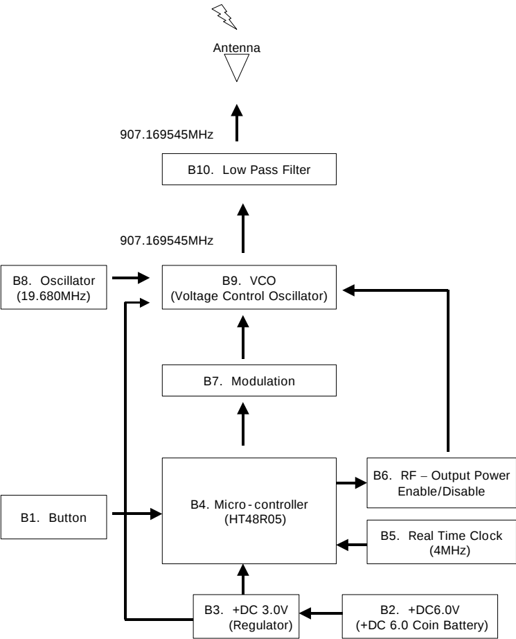
N99J1WPLL4R Block Diagram (B1<Block1> ~ B10<Block10>)
