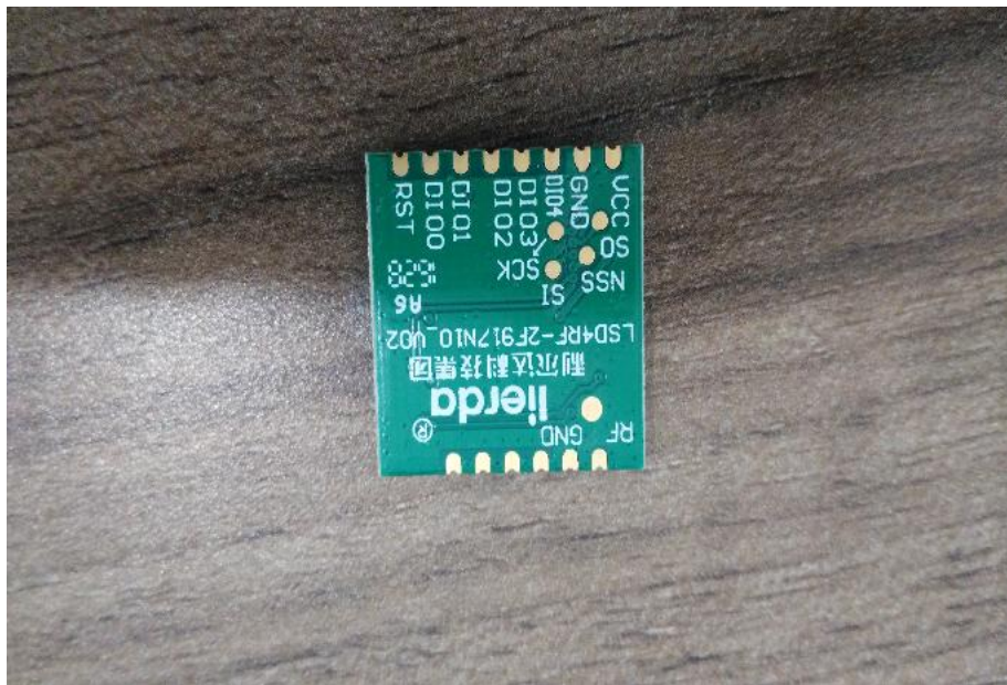
(1) EUT Photo
