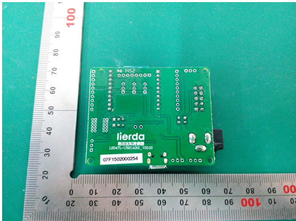
EUT with Base board Back side
