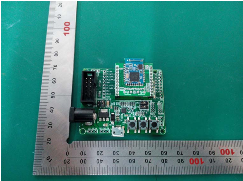
EUT with Base board front side
