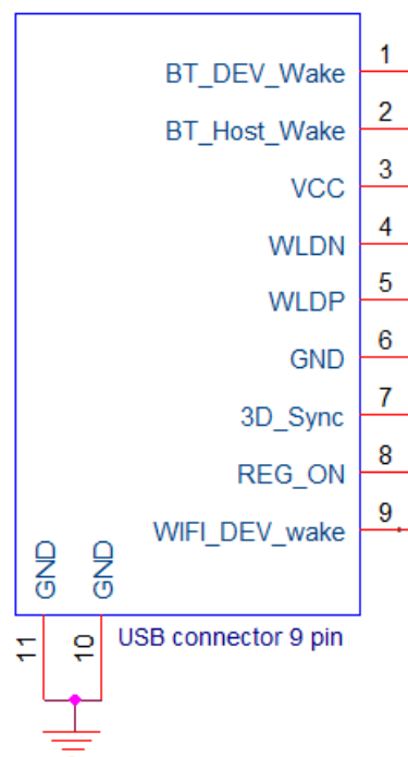
Figure 2: Pins Configuration
