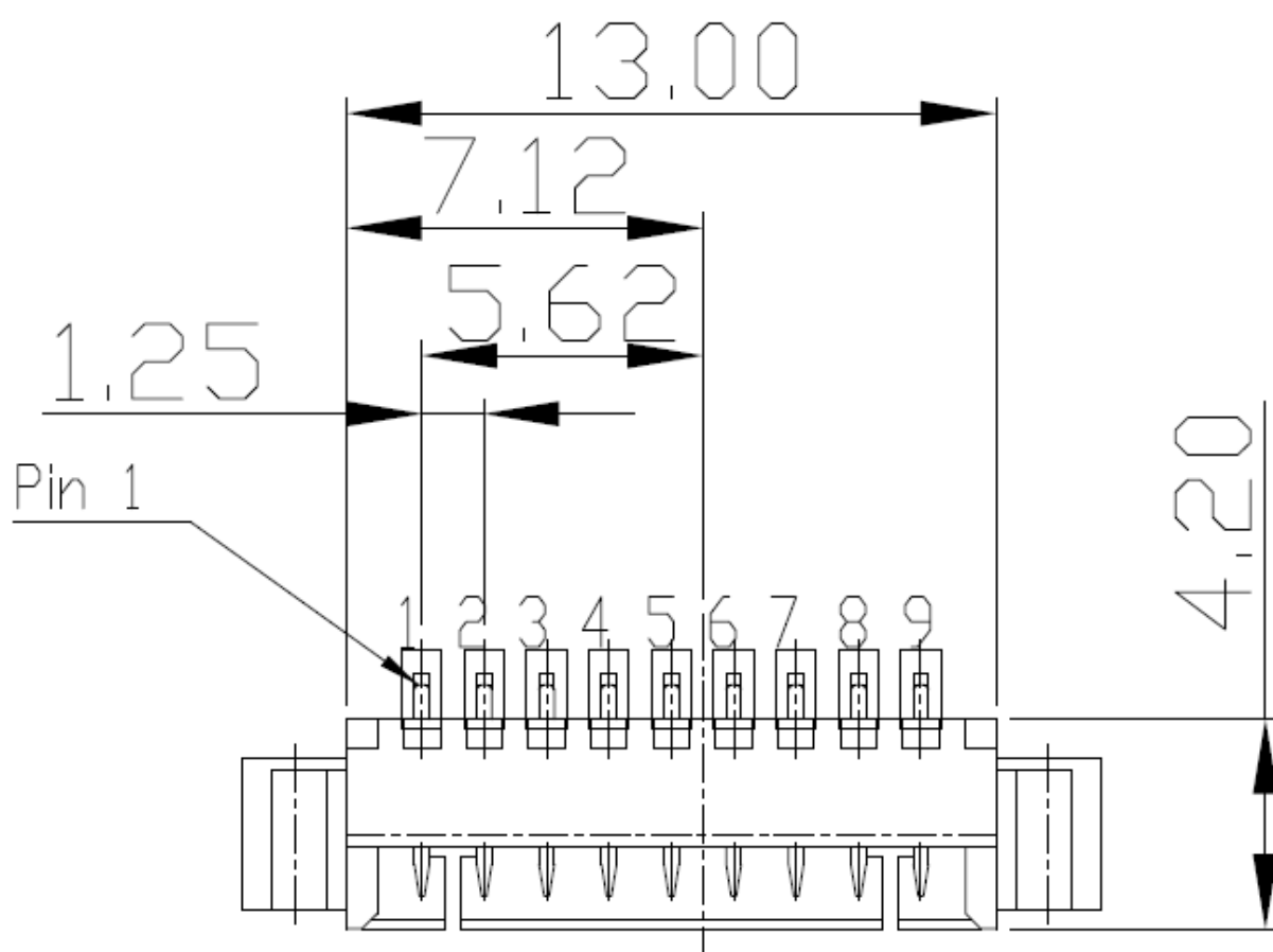
Figure 1: WTB Connector Layout
