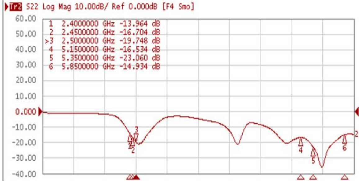
Figure 1 Return Loss
