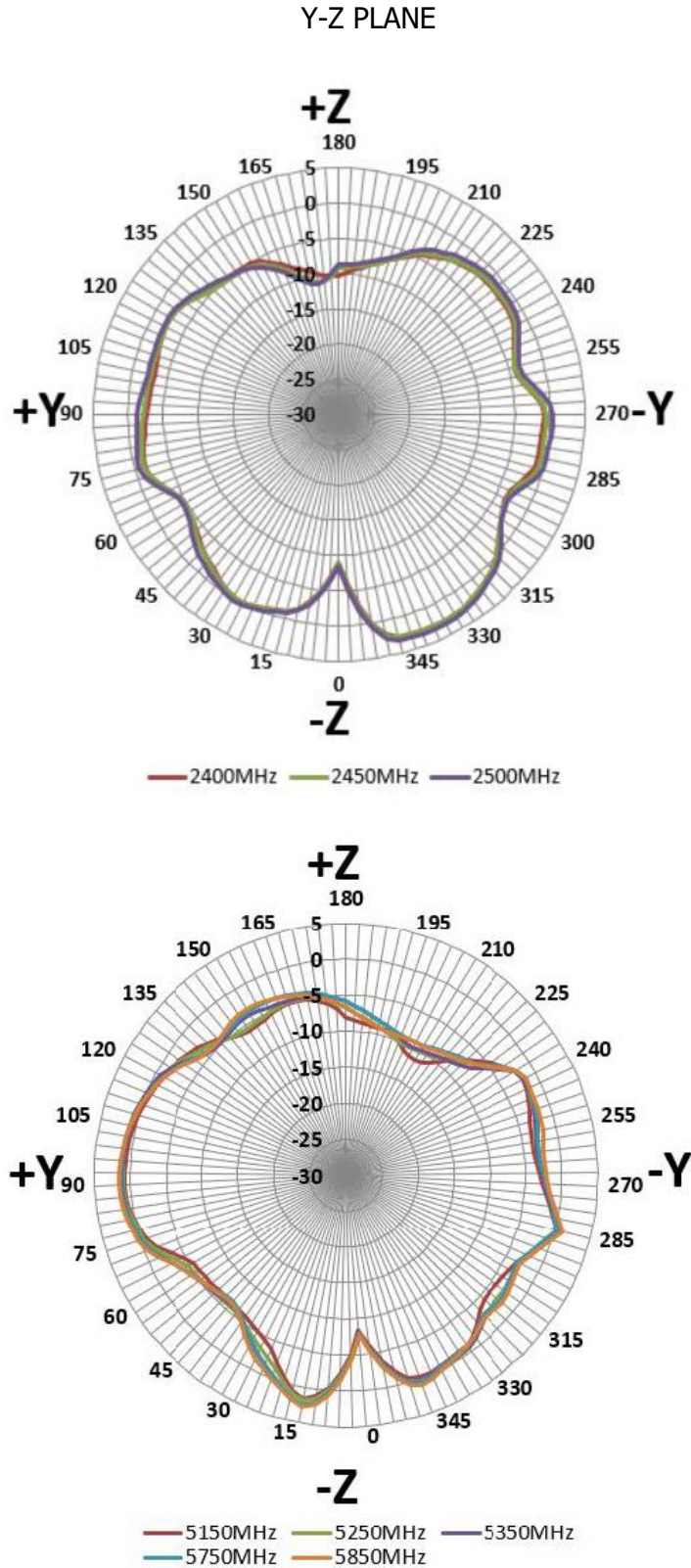
Figure 3 Radiation Patterns in Wi-Fi Dual Band.
