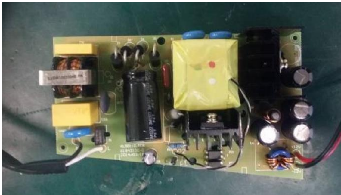
37.8W Power board using in K-5401
