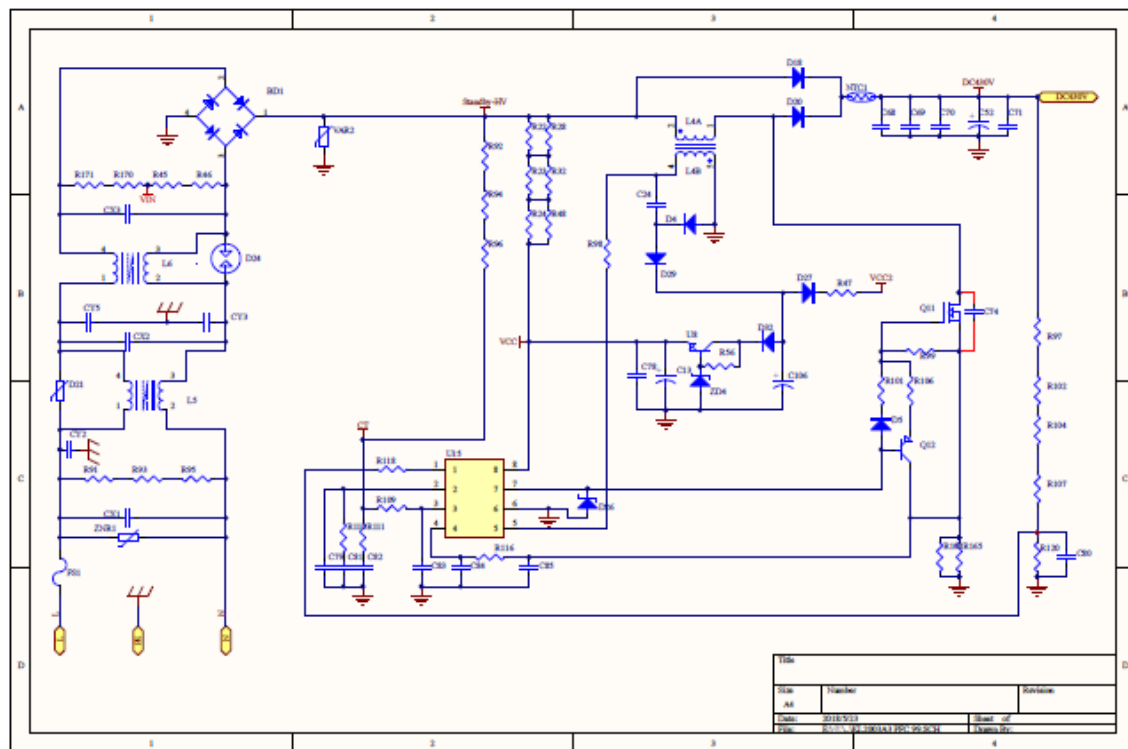
Schematics of 218W Power board
