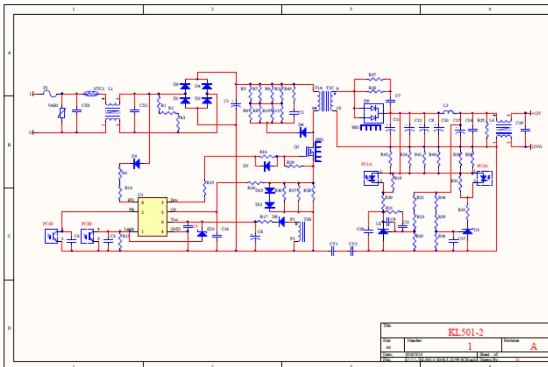
Schematics of 37.8W Power board
