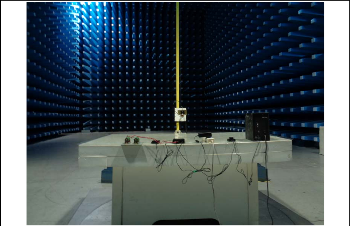
Radiated Spurious Emissions Test Setup Below 1GHz
