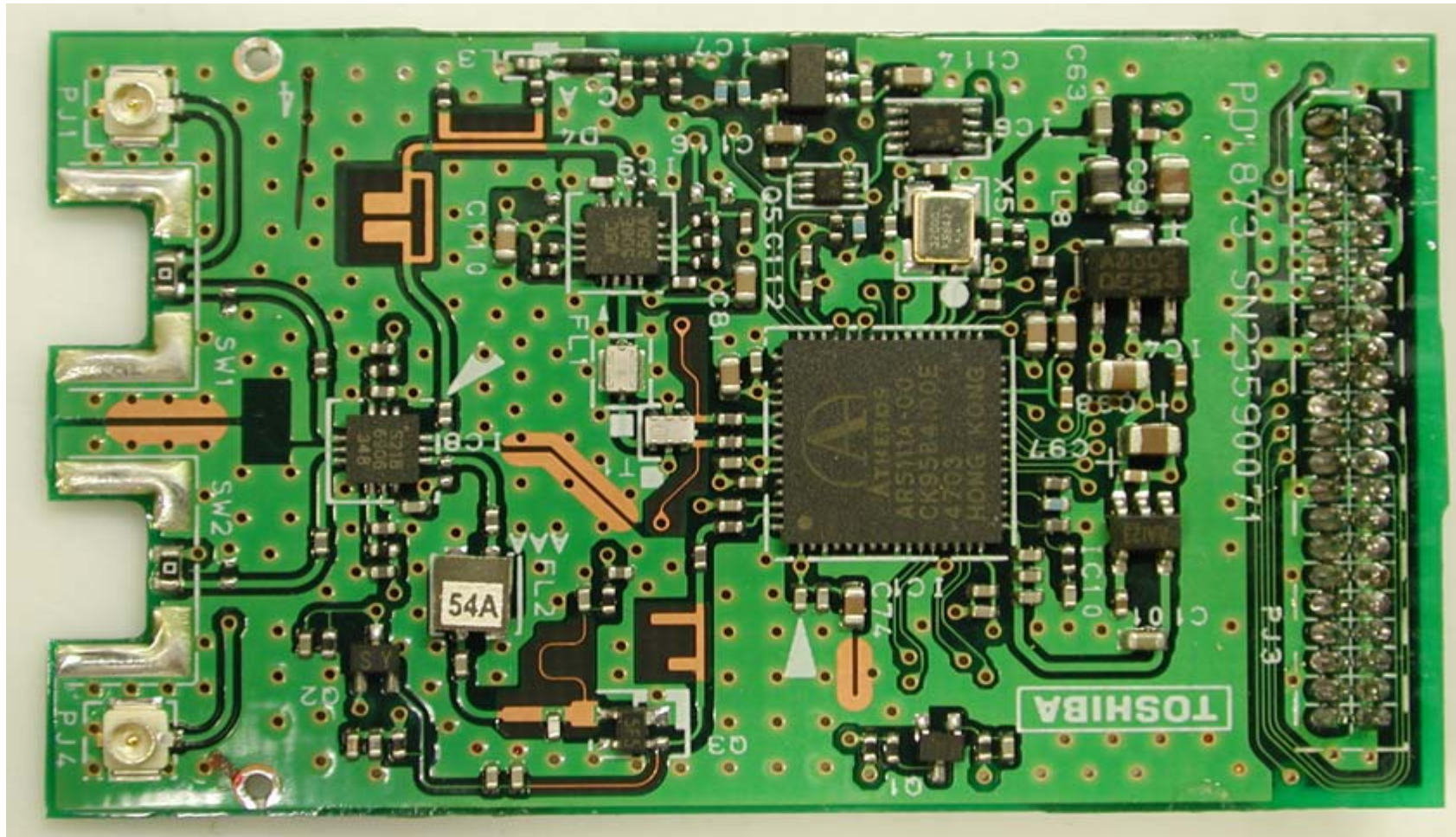
Module picture without shielding
