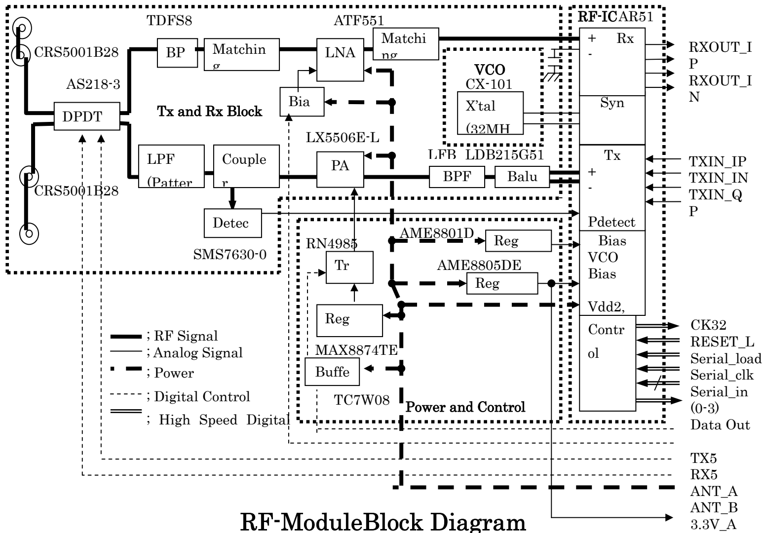
Block Diagram for Model WVM-1101
