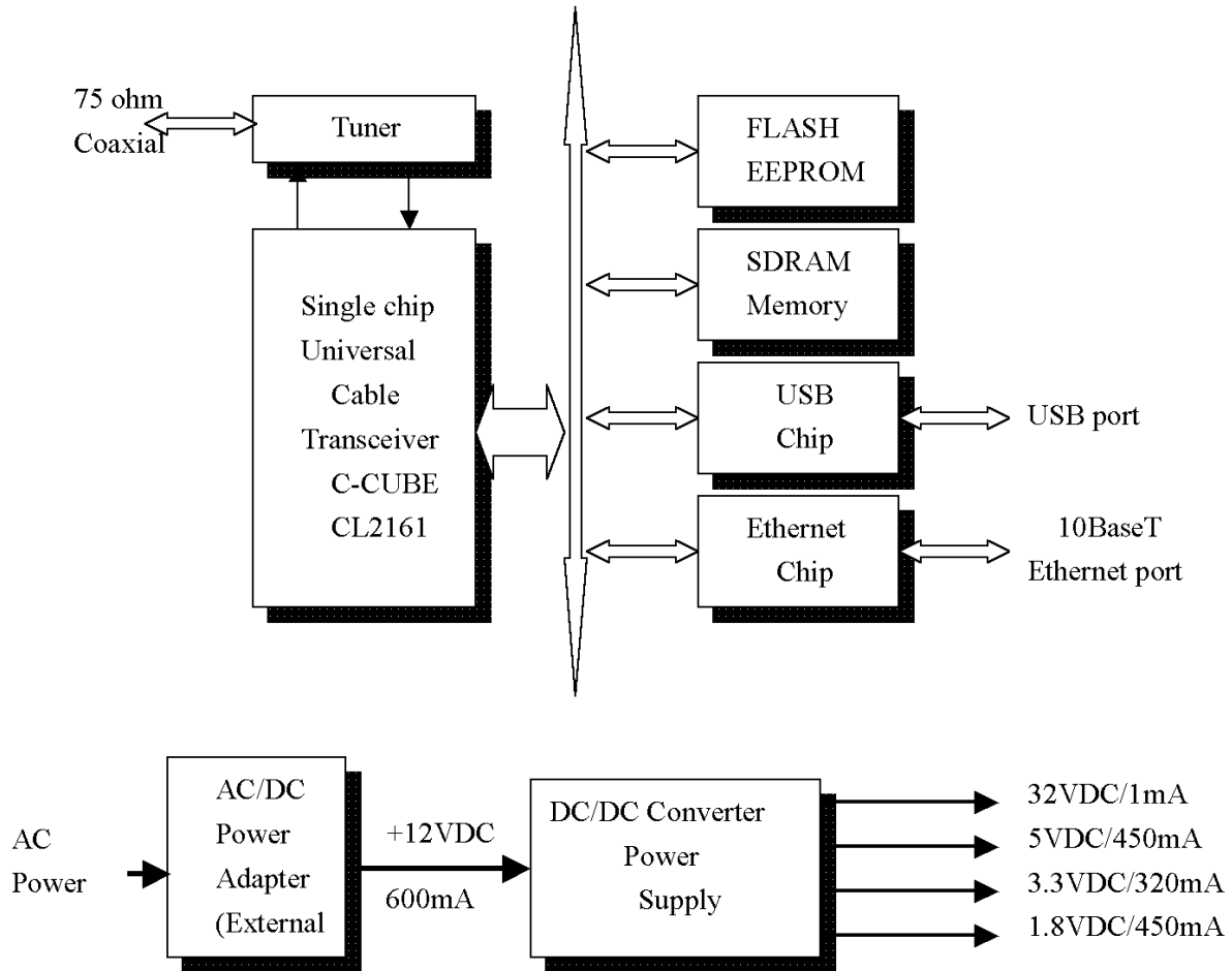
Block diagram of External USB cable modem
