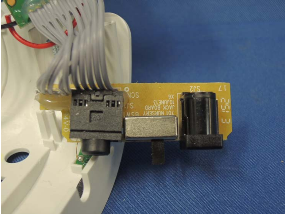
Baby Unit Jack Board front side
