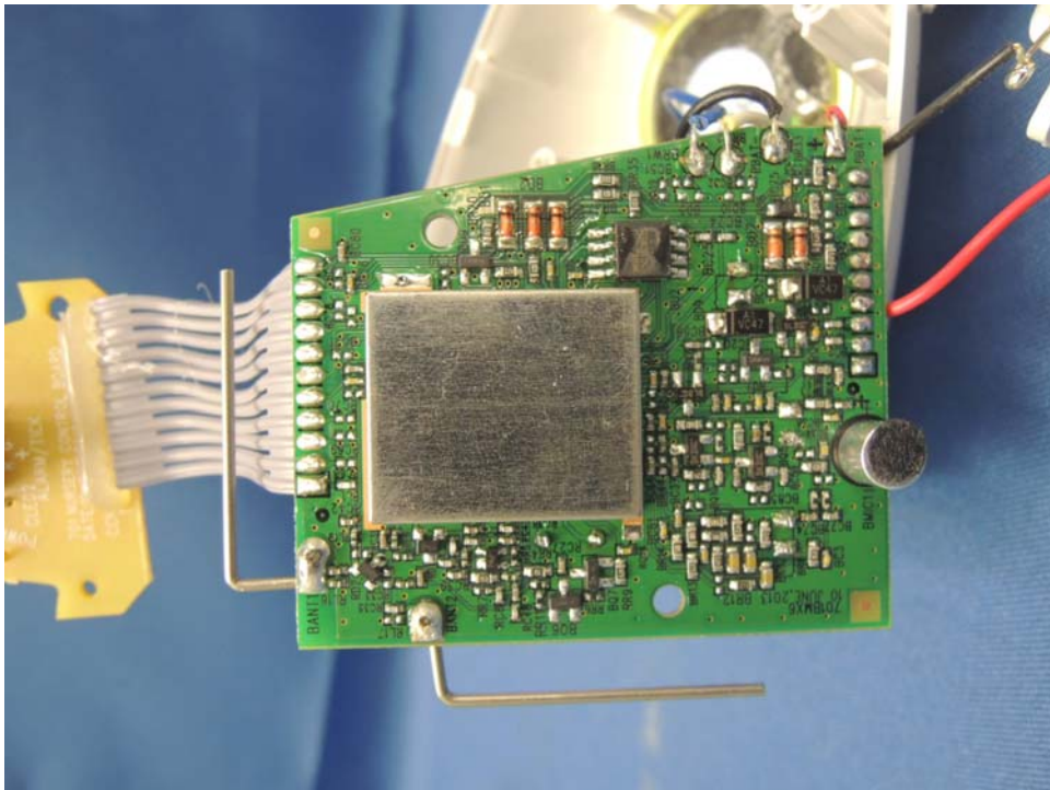
Baby Unit Main PCB comp side (1)
