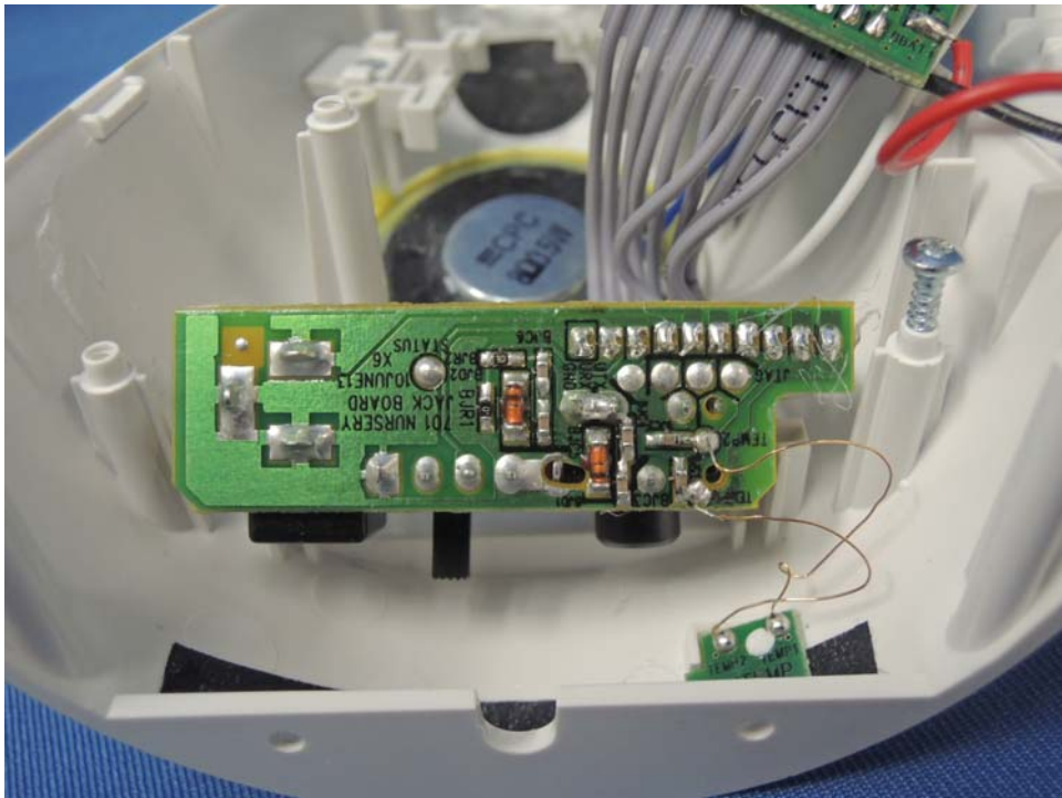
Baby Unit Jack Board rear side
