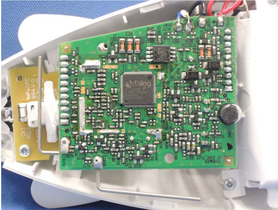
Baby Unit Main PCB comp side (2)
