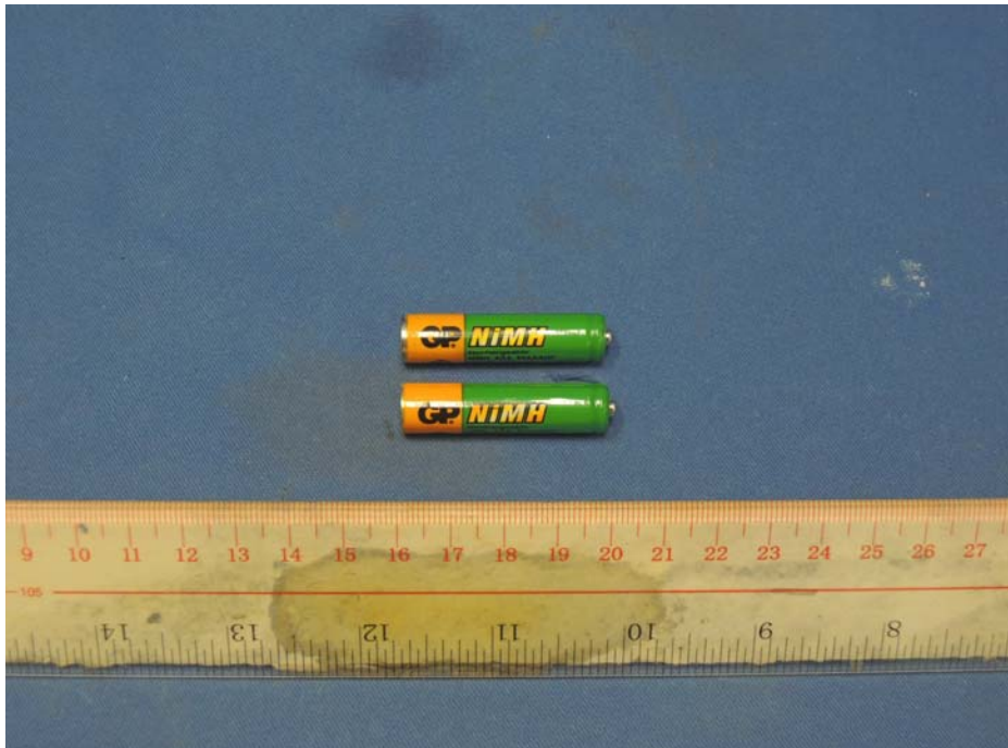
Figure 3 – 2 x 1.2V 600mAH GP Ni-MH rechargeable battery
