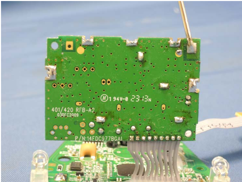
Baby Unit Oscillator PCB solder side
