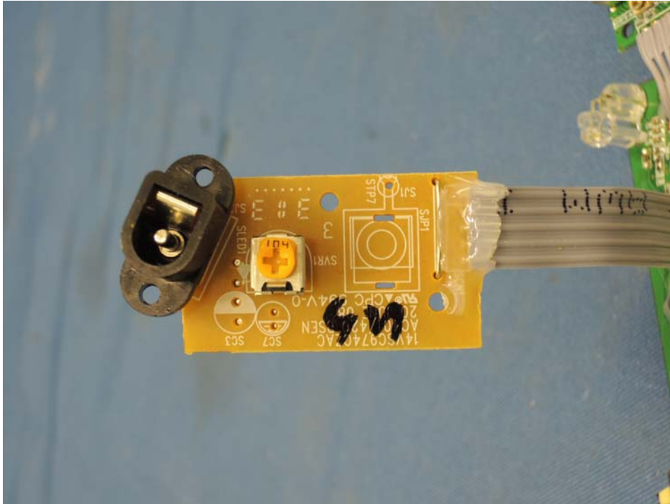
Baby Unit AC Jack front side
