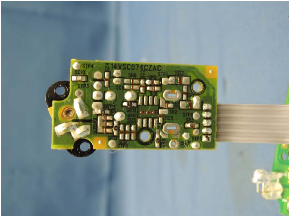
Baby Unit AC Jack rear side
