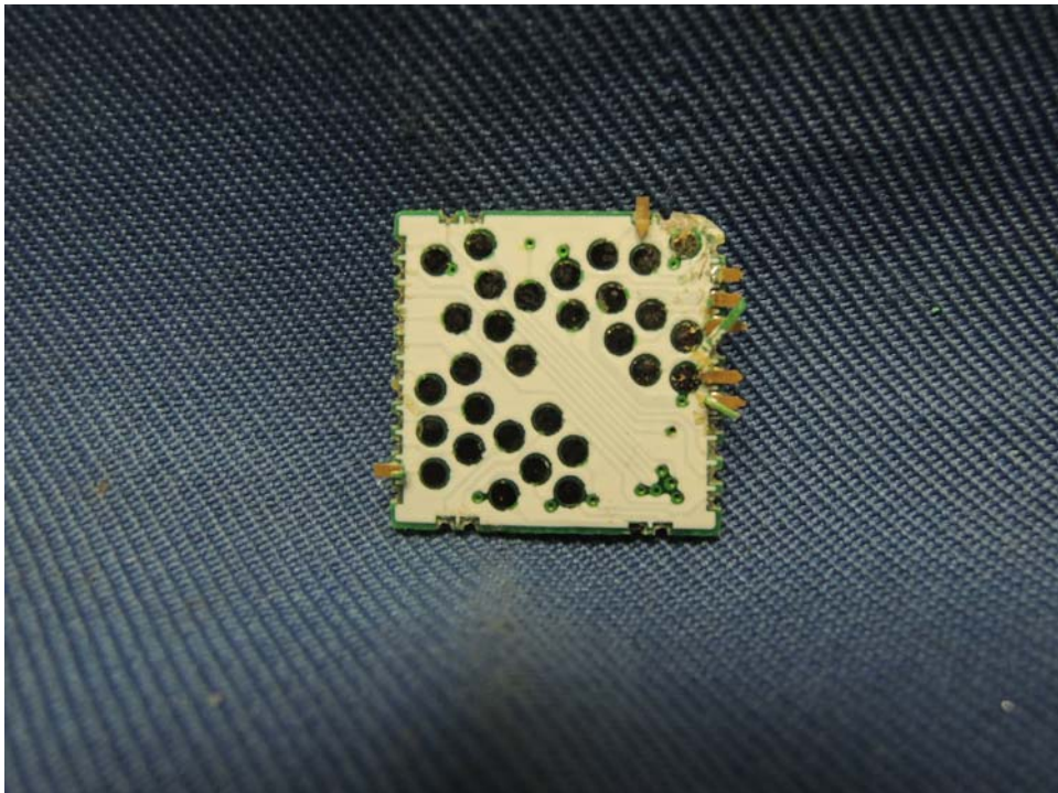
Baby Unit MCU PCB rear side
