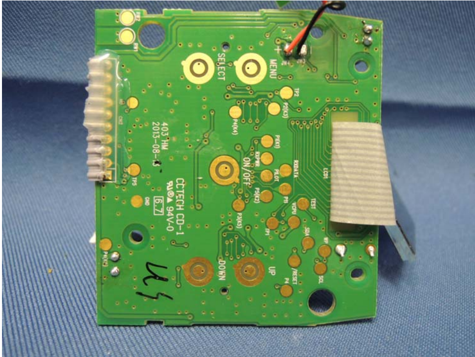
Parent Unit Main PCB solder side (View 3)
