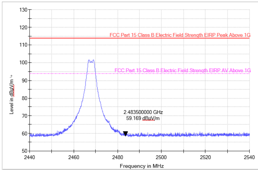
Electric Field Strength 1-18GdBuV TX EIRP
