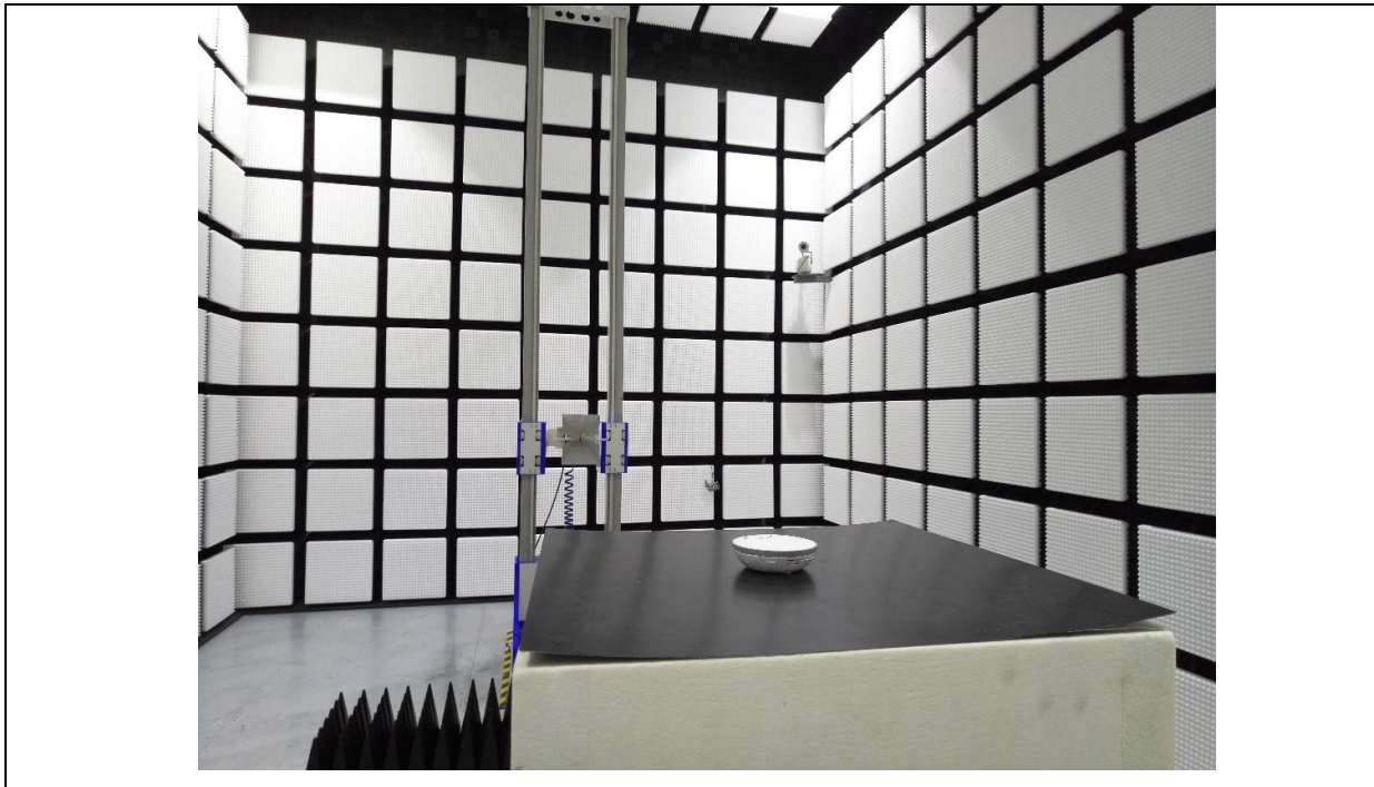
Spurious radiated emissions (above 1G)
