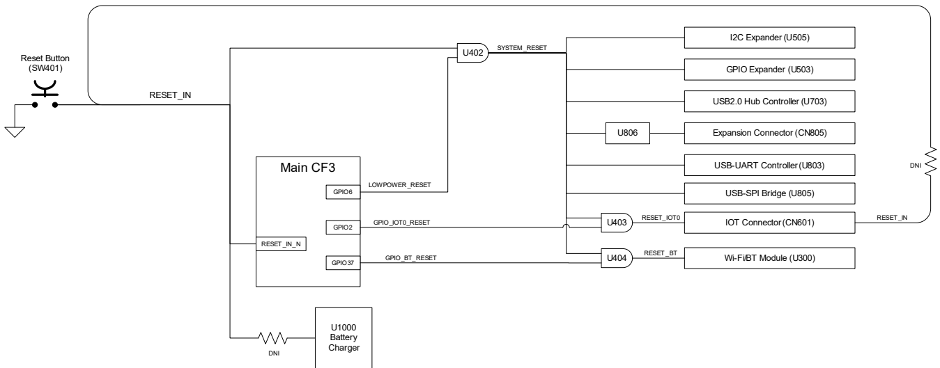
Figure 2-27: Reset Methods
