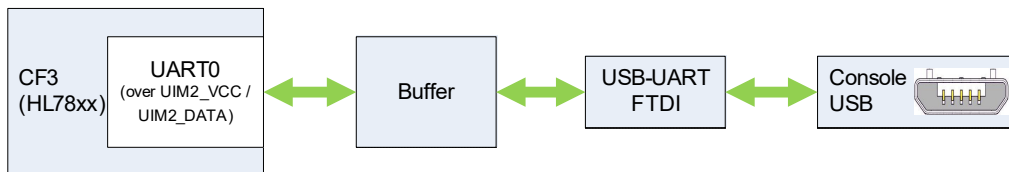
Figure 2-19: UART0 Configuration
