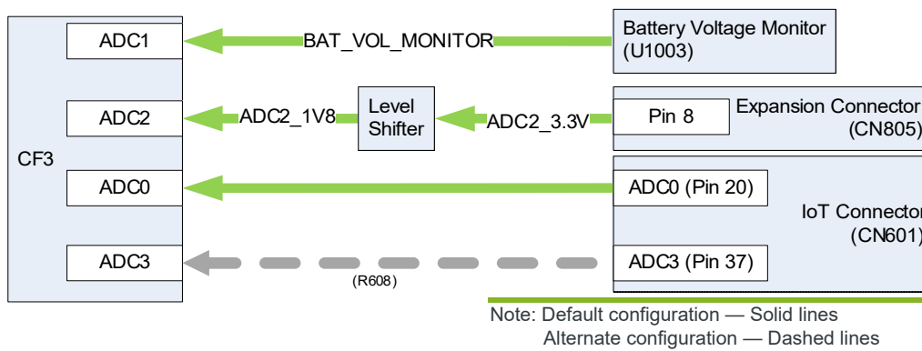
Figure 2-7: ADC Configuration
