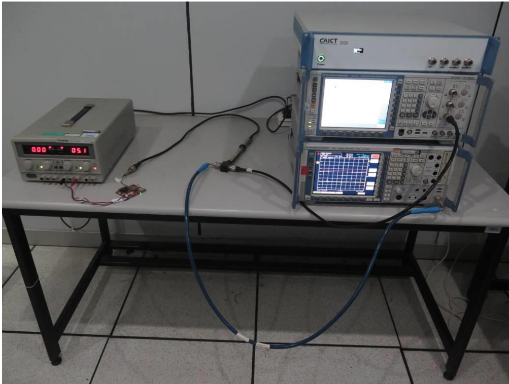
Pic.1 Conducted test set-up
