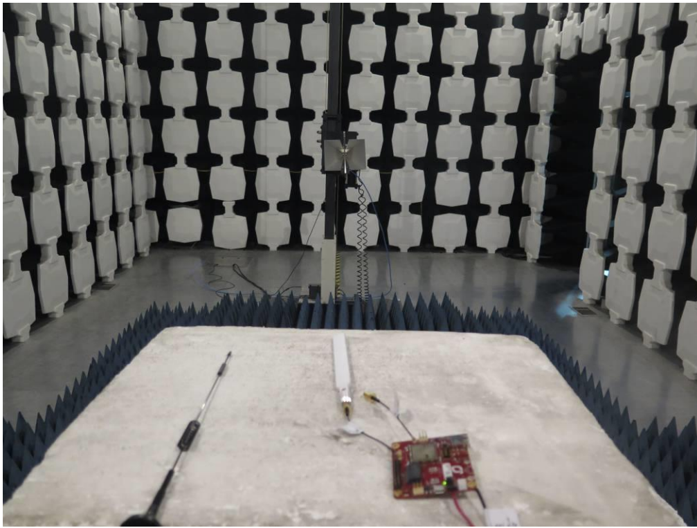
Pic.3 Radiated test set-up 2
